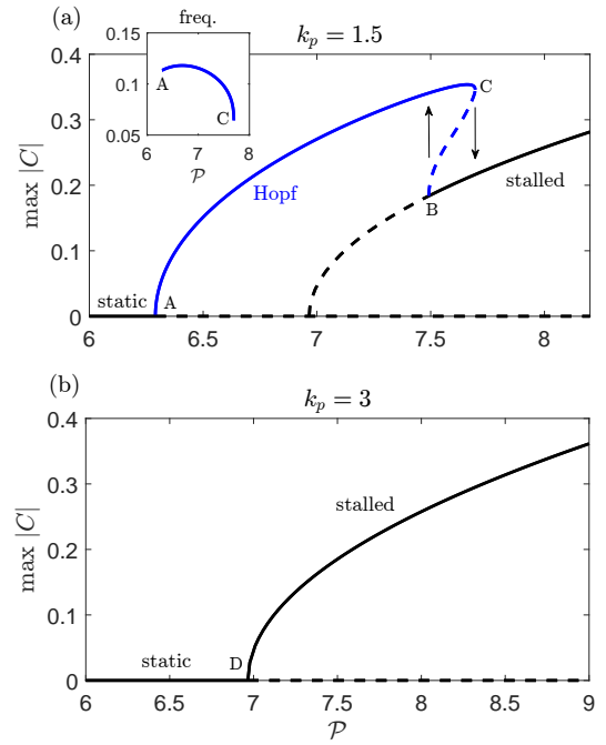
FIG. 14. Two typical bifurcation diagrams for an elastically confined AP when the stiffness k_p < k_p^* (a) and when k_p > k_p^* (b). The continuation of the Hopf bifurcation is shown in blue while supercritical pitchfork (second order phase transitions) are shown in black. In inset of (a), we show the frequency (inverse of the period) of the stable Hopf oscillations as a function of the continuation parameter. The dashed lines are linearly unstable branches while full lines are stable. Arrows indicate the discontinuous transitions. The capital letters are related to the phase diagram shown on Fig. 13. Parameter \mathcal{L} = 2 .
