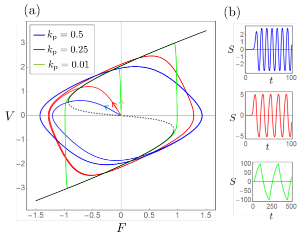
FIG. 15. Dynamics of the oscillations when the stiffness k_p of the environment starting from the initial state (S_0, C_0) . (a) represents the trajectories of the oscillating particle in the phase space (k_p S, \dot{S}) for three different stiffnesses. We superimpose in black color the V-F curve obtained for a fixed force (Section. IV). On (b) we show the related particle position steady state oscillations. Parameters \mathcal{L} = 2 and \mathcal{P} = 6.5 .
