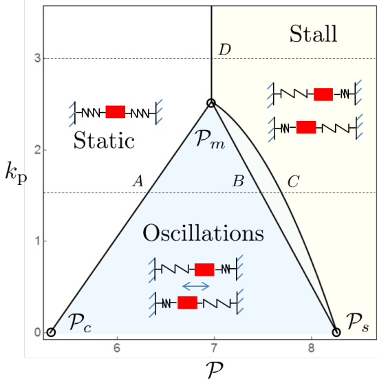
FIG. 13. Stability diagram of an AP confined by harmonic springs depending on the contractility and environment stiffness. Note the region of coexistence (metastability) between the oscillations and stall phases where the two types of solutions coexist. The two thin dashed lines and associated capital letters are related to the bifurcation diagrams shown on Fig.14. Parameter \mathcal{L} = 2 .
