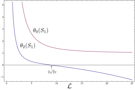
FIG. 20. Eigenvalues \theta_0 and \theta_2 as a function of \mathcal{L} for the first static branch S_1 .
