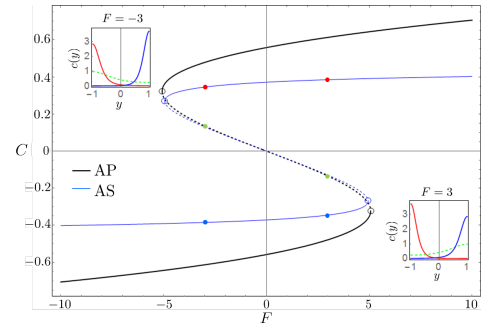
FIG. 8. Comparison of the global polarity C as a function of the force in AS (blue) and AP models (black). The dashed parts of the C-F curve correspond to unstable regimes. We show in inset the motor concentration in the AS case at forces F = -3 and F = 3 . The red profiles have a positive polarity while the blue profiles have a negative polarity. A central symmetry transforms a red (resp. blue) profile at a positive force into a blue (resp. red) profile at a negative force. The green profiles are related to the unstable branch. Parameters \mathcal{L} = 2 and \mathcal{P} = 9 .
