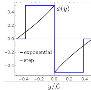
FIG. 1. Two interaction kernels \phi(y) : black line is the exponential kernel of this paper and blue line is the kernel used in [37]. Parameter \mathcal{L} = 2 .
