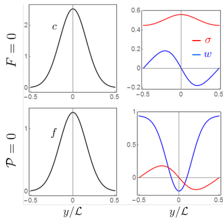
FIG. 2. Non local response of the stress field (see (9)) and the velocity field (see (10)) to a contractility distribution with no external force (first row, F = 0 and \mathcal{P} = 1 ) and to a force distribution with no contractility (second row, \mathcal{P} = 0 and F = 1 ). Parameter \mathcal{L} = 2 .
