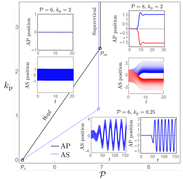
FIG. 12. Linear instability thresholds of the static solution in the AP and AS case. We show in insets some typical static, stalled and oscillatory dynamics for the AP and AS case. The intensity of the coloring is proportional to the motor concentration for the AS case. Parameter \mathcal{L} = 2 .
