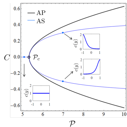
FIG. 4. Spontaneous polarization in AS and AP models when contractility increases above the critical threshold \mathcal{P}_c . We show in insets typical concentration profiles of molecular motors along the bifurcated branches in the AS model. Parameter \mathcal{L} = 2 .
