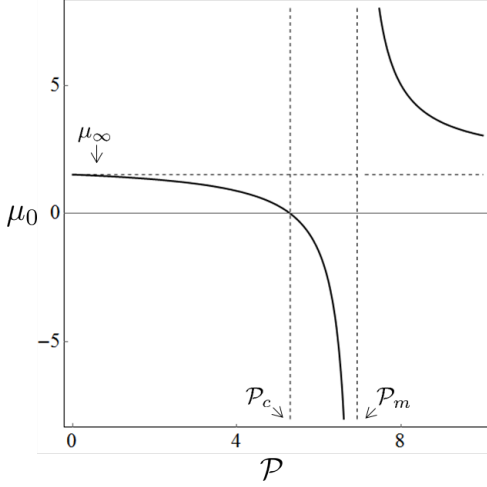
FIG. 18. Effective frictional viscosity at the origin of the V-F curve, \mu_0 as a function of contractility parameter \mathcal{P} . Parameter \mathcal{L} = 2 .
