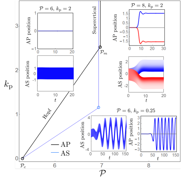
FIG. 12. Linear instability thresholds of the static solution in the AP and AS case. We show in insets some typical static, stalled and oscillatory dynamics for the AP and AS case. The intensity of the coloring is proportional to the motor concentration for the AS case. Parameter \mathcal{L} = 2 .
