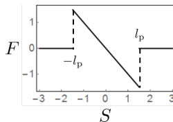
FIG. 16. Scheme of the harmonic confinement force with a threshold.
