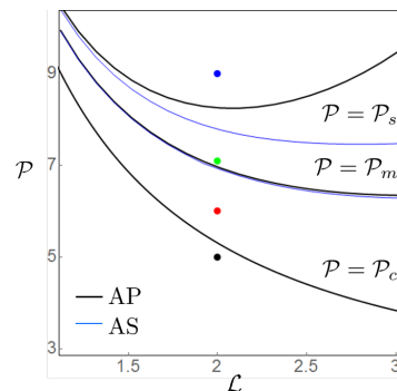
FIG. 5. Dependence of three contractility thresholds \mathcal{P}_c , \mathcal{P}_m and \mathcal{P}_s on parameter \mathcal{L} representing the segment length. The value of \mathcal{P}_c is the same in both the AS and AP models by construction. The color dots are choices of parameters related to the V-F relations shown in Fig. 6.
