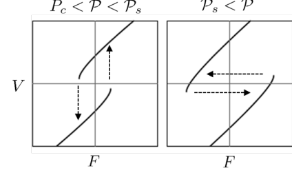
FIG. 7. Schematic representation of the single and double hysteretic V-F relations.
