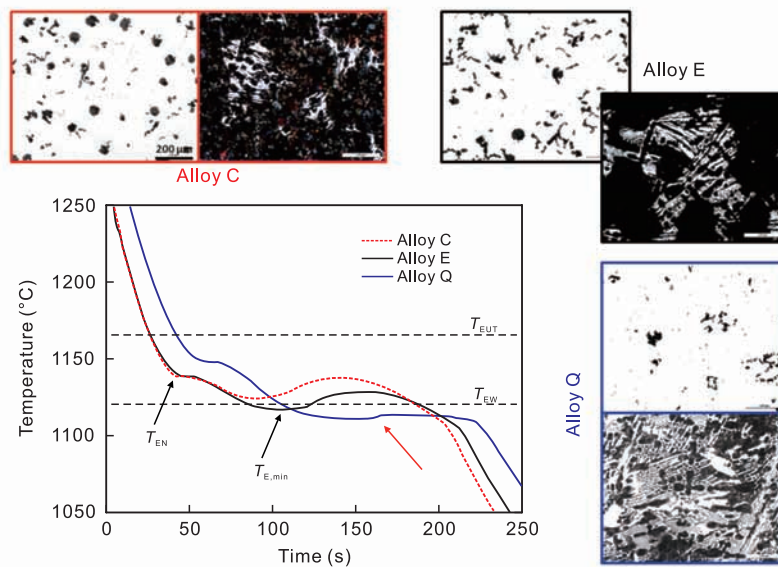
Fig. 1: Experimental cooling curves of the three selected samples ( C_{uninoc} , E_{uninoc} and Q_{uninoc} ) and related optical micrographs before and after nital etching. The scale of the micrographs is the same for all and is shown in the upper left one
