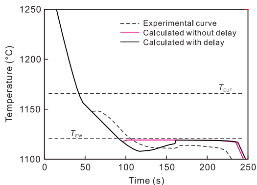
Fig. 4: Comparison of experimental and calculated cooling curves for the uninoculated Alloy Q. Ledeburite appearance was calculated either without (thin red solid line) or with (thick black solid line) a time delay
