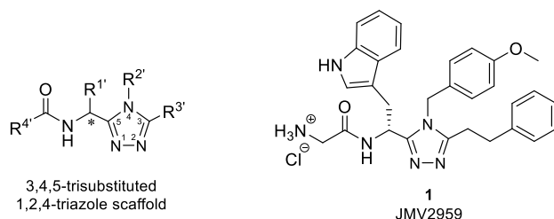
Figure 1. Structure of the 3,4,5-trisubstituted 1,2,4-triazole scaffold and compound 1 (JMV2959)
