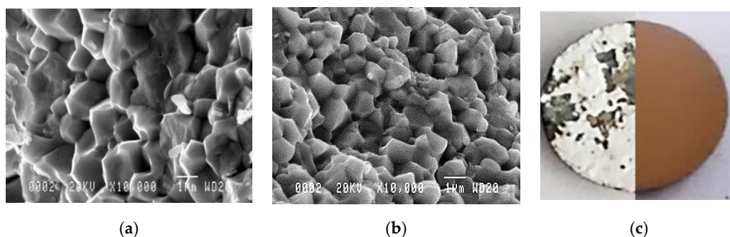
Figure 8. SEM images of fractured PZT ceramics sintered by spark plasma sintering (SPS) at 875 °C without a sintering aid: (a) Without a protective layer and (b) with \text{SrCO}_3 . (c) Elimination of the \text{SrCO}_3 layer by etching or polishing.
