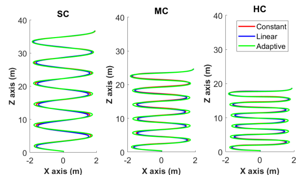
Figure 2: Average path (after filtering the data) followed by participants depending on control law and curvature type.
