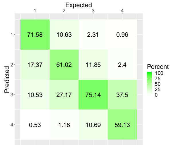
Figure 9: Confusion matrix for “HMD sensors” (Expected and predicted classes) in the “All physio+perf” using NSF normalization setup.
