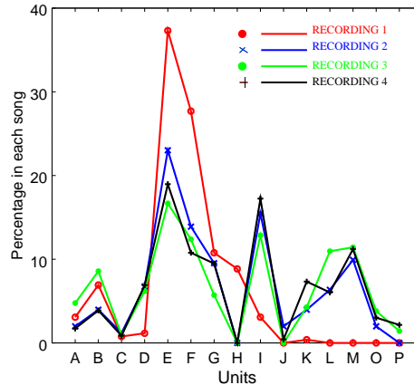
Figure 7. Percentage of each unit in the four song occurrences of recording #1 from Abrolhos archipelago, 2000 (colors are red, blue, green and black for song occurrences 1,2,3,4 respectively). The first occurrence of the song in the recording (see figure 4), in red in this figure is quite different from the other occurrences in term of its units, due to boat noise that prevented an accurate identification of several units.
