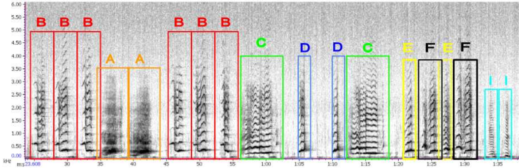
Figure 1. Time (min:sec) / frequency (kHz) representation of an extract of recording #3 (from Abrolhos Archipelago 2000), 1024 point FFTs, Hann window, 43.1 Hz resolution and 50% overlap. Unit transcription into letters is signaled above the boxes
