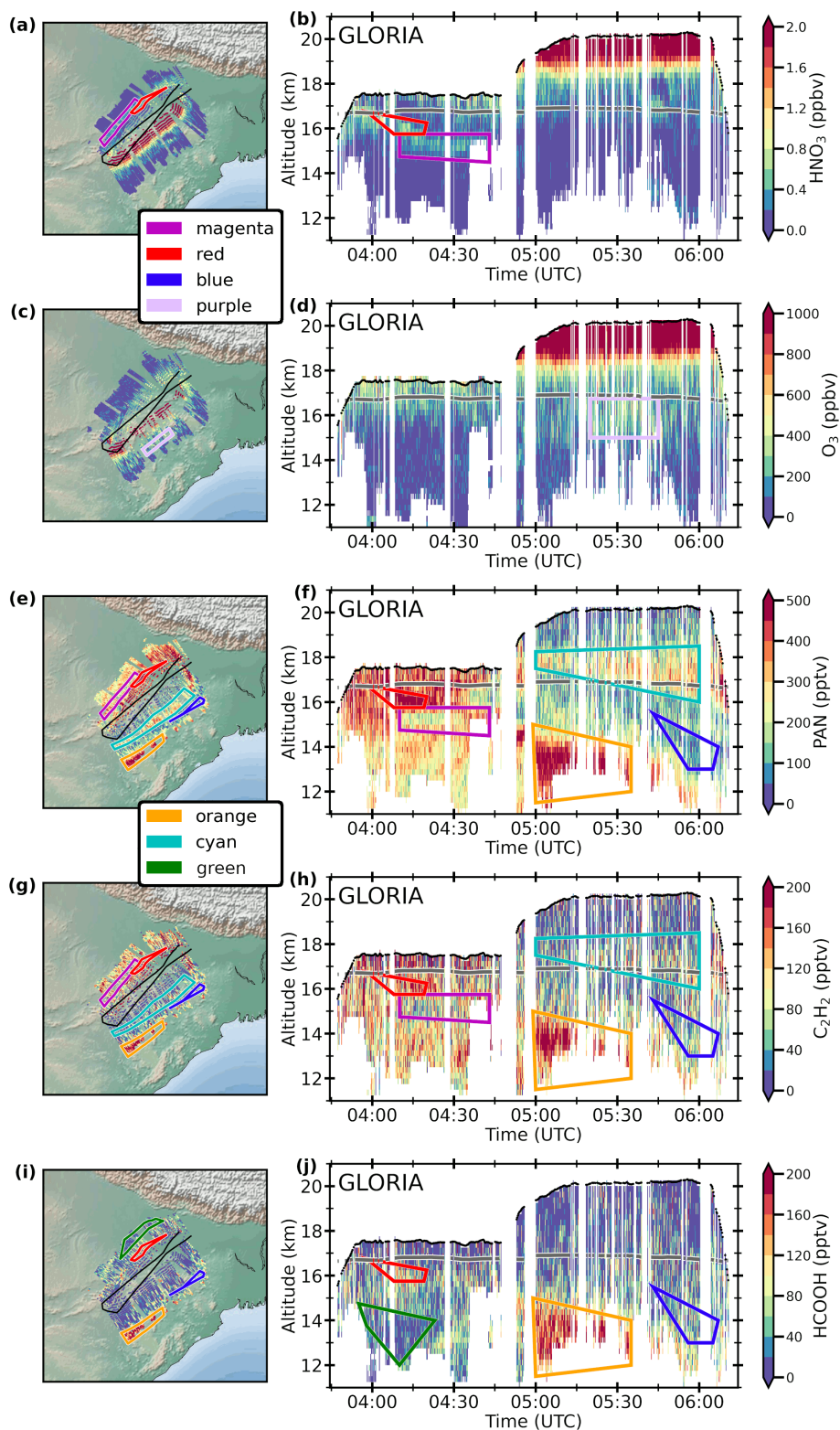
Figure 2. Horizontal (a, c, e, g, i) and vertical (b, d, f, h, j) distributions of GLORIA measurements of (a–b) \text{HNO}_3 , (c–d) \text{O}_3 , (e–f) PAN, (g–h) \text{C}_2\text{H}_2 , and (i–j) HCOOH for the StratoClim flight on 31 July 2017. The black line in the maps and cross sections shows the flight path and the dark gray line (on the cross-section plots only) the 380 K potential temperature isentrope as approximate tropopause altitude. Colored boxes mark air masses of interest, discussed in the following sections. The maps are centered on the Indian subcontinent.
