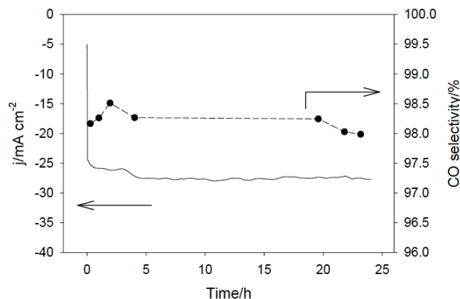
Figure 2. Current density (left axis) and CO selectivity (right axis) during a 24 h electrolysis at E = -0.78 V vs RHE in 0.5 M NaHCO 3 electrolyte solution.
