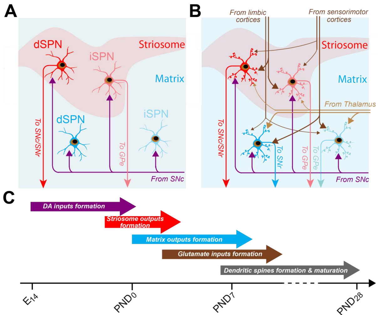
Figure 2: Establishment and maturation of the developing striatum. A-B: Schematics depicting the sequential maturation of the striatum. A: Dopaminergic inputs and axonal projections of striosomal SPNs develop principally between E14 and birth (PND 0 ). B: During the first postnatal week, matrix SPNs make connections with their targets (the SNr and the GPe) and glutamatergic inputs from the cortex and thalamus are formed. Between the first and fourth postnatal weeks, the striatal microcircuit becomes fully functional with a strengthening of glutamatergic inputs and the formation and maturation of SPN dendritic spines. C: Timeline showing the different key steps involved in the maturation of the developing striatum.
