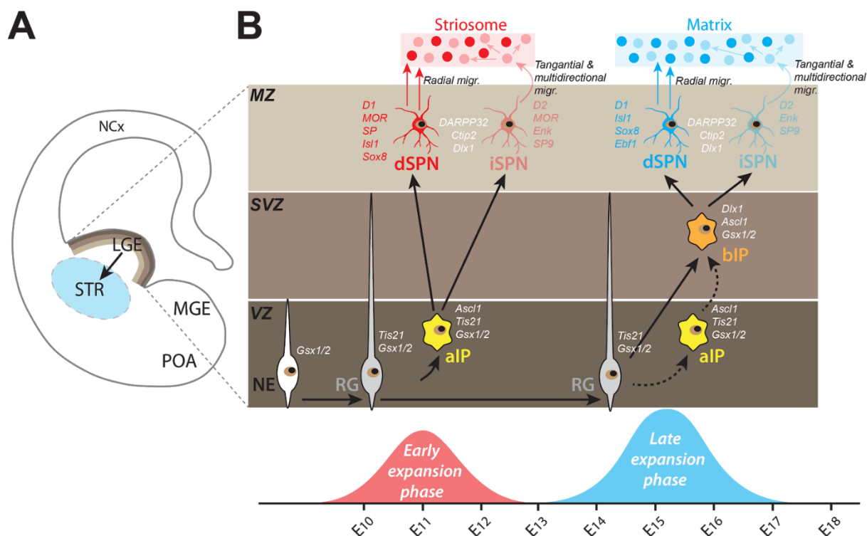
Figure 1: Current model of embryonic mechanisms underlying striatal architecture and the ontogenesis of SPNs. A: Schematic representation of a coronal hemisection of the developing brain in which are represented the neocortex (NCx), striatum (STR), lateral ganglionic eminence (LGE), medial ganglionic eminence (MGE) and the preoptic area (POA). B: Enlargement of the LGE region indicating the different expansion phases of neuroepithelial (NE) cells leading to the formation of striosomal and matrix striatal compartments. In the early (E10-E12.5) expansion phase, NE cells give rise to radial glial (RG) cells that generate apical intermediate precursors ( aIP ), which in turn give rise to striosomal dSPNs and iSPNs. A second wave of expansion takes place between E13 and E17, during which RG cells give rise directly or indirectly through aIP (dashed arrows) to basal intermediate precursors ( bIP ) which will produce matrix dSPNs and iSPNs. While striosomal and matrix dSPNs eventually reach their final destination in the developing striatum following radial migration, iSPNs reach their targets through a tangential and multidirectional migration process.
