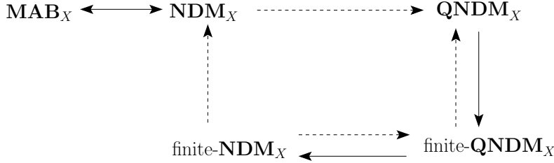
Figure A.4: Relations between semantics for the language \mathcal{LANG}_{LDA} . An arrow means that satisfiability relative to the first class of structures implies satisfiability relative to the second class of structures. Full arrows correspond to the results stated in Lemmas 5, 6 and 7. Dotted arrows denote relations that follow straightforwardly given the inclusion between classes of structures.
