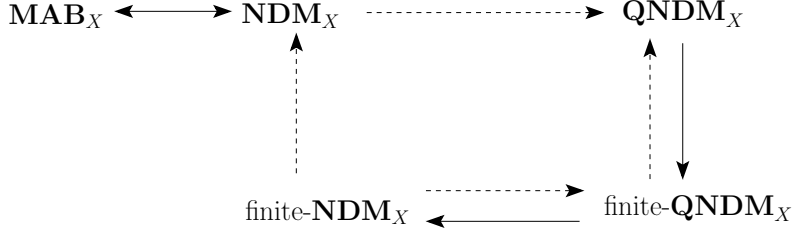
Figure A.4: Relations between semantics for the language \mathcal{LANG}_{\text{LDA}} . An arrow means that satisfiability relative to the first class of structures implies satisfiability relative to the second class of structures. Full arrows correspond to the results stated in Lemmas 5, 6 and 7. Dotted arrows denote relations that follow straightforwardly given the inclusion between classes of structures.
