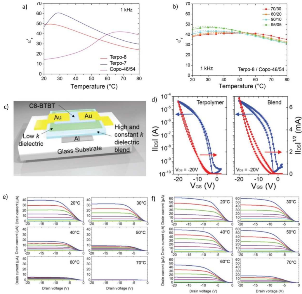
Figure 2. a), b) Dielectric spectroscopy at 1kHz of a) P(\text{VDF-co-TrFE}) copolymer compared to P(\text{VDF-ter-TrFE-ter-CTFE}) terpolymers b) comparison of terpolymer copolymer blends. c) Schematic representation of OFET architecture. d) Transfer characteristics in saturation regime ( V_{DS} = -20\text{ V} ) of OFET with either terpolymer or terpolymer-copolymer blend as gate dielectric layer. e) output characteristics at different operating temperature of OFETs with terpolymer and f) with the blend system showing improved thermal stability. Reproduced with permission from [17]. Copyright (2020)
