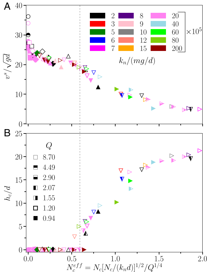
Fig. 3. The flow is controlled by the dynamic “effective” adhesive force. Variation of the free surface velocity ( v^s/(gd)^{1/2} ) (A) and the thickness of the plug ( h_c/d ) (B) with the dynamic “effective” adhesive force N_c^{eff} at \theta = 29^\circ for different N_c (different symbols; see Fig. 2 for the key), different k_n (different colors), and different Q (different symbol pattern). The dashed line indicates the transition from a plug-less to a plug-full velocity profile.
