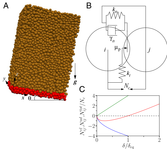
Fig. 1. Simulation of flow of cohesive grains down a rough inclined plane. (A) Snapshot of a simulation, showing the flow of particles (in brown) under gravity \mathbf{g} over a bumpy base (in red) inclined at an angle \theta . (B) Depiction of the visco-elastic, frictional, and adhesive interactions between the particles using a spring-dashpot model with a frictional slider and an interparticle adhesion N_c . (C) The nonviscous normal contact forces normalized by the interparticle adhesion as a function of the normalized overlap \delta/\delta_{eq} : elastic part N_{ij}^{el} (green), adhesive part N_{ij}^{ad} (blue), and the sum of the two N_{ij}^{tot} = N_{ij}^{el} + N_{ij}^{ad} (red). See the main text for \delta_{eq} .
