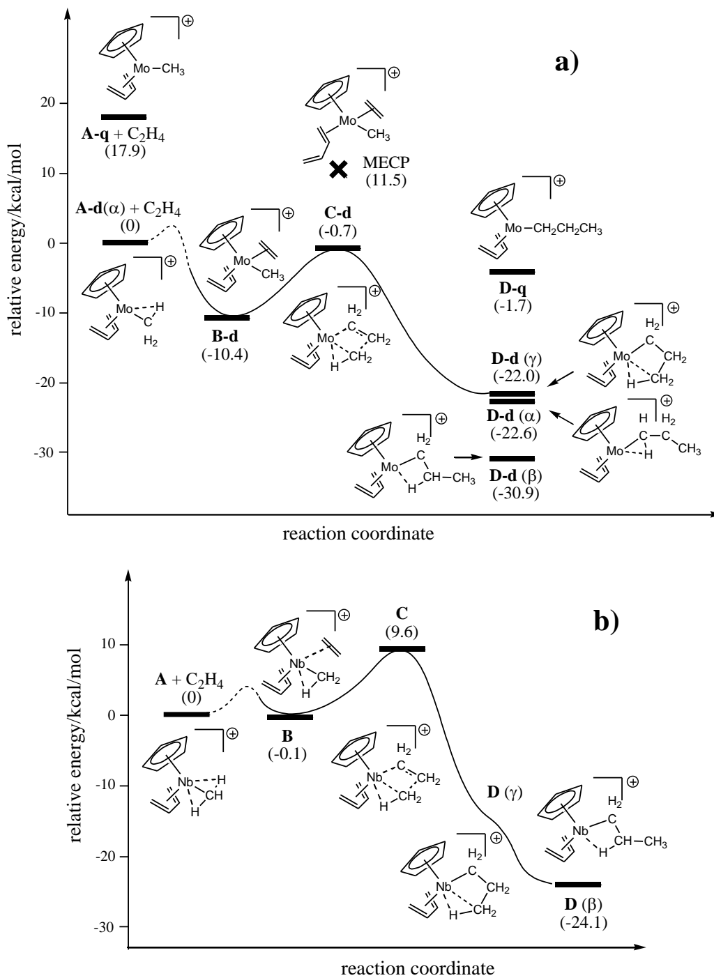
Figure 2. Energy diagram and key structures for the ethylene insertion reaction into the Mo-CH 3 bond of [CpMo(η 4 -C 4 H 6 )(CH 3 )] + .
