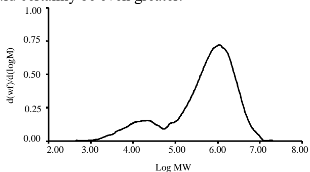
Figure 1. GPC trace of polyethylene obtained from run 10 (Table 2). Solvent = 1,2,4-trichlorobenzene. T = 135^{\circ}\text{C} .
