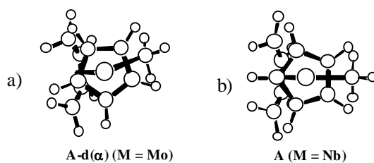
Figure 3. Top views of the optimized geometries for [CpM(C 4 H 6 )(CH 3 )] + (a: M = Mo; b: M = Nb).
