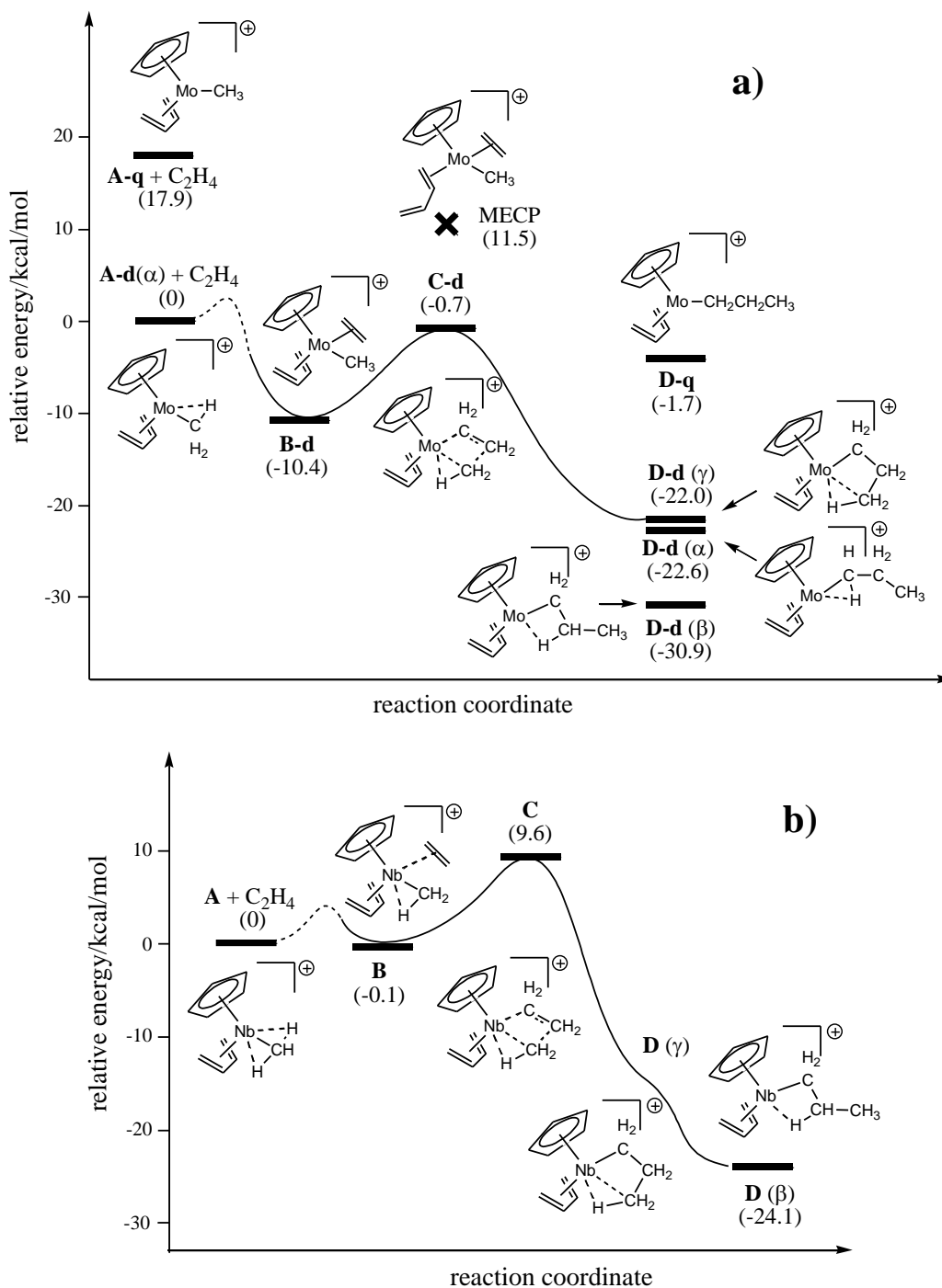
Figure 2a) was not calculated. Previous studies have shown that this step proceeds without an enthalpic barrier for metallocene type systems, even when stronger \beta -agostic interactions are
