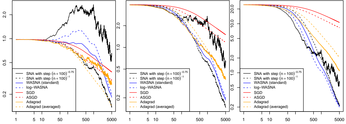
Figure 4: (Logistic regression with correlated Gaussian variables) Mean-squared error of the distance to the optimum \theta with respect to the sample size for different initializations: \theta_0 = \theta + r_0 U , where U is a uniform random variable on the unit sphere of \mathbb{R}^d , with r_0 = 1 (left), r_0 = 2 (middle) or r_0 = 5 (right). Each curve is obtained by an average over 50 different samples (drawing a different initial point each time).
