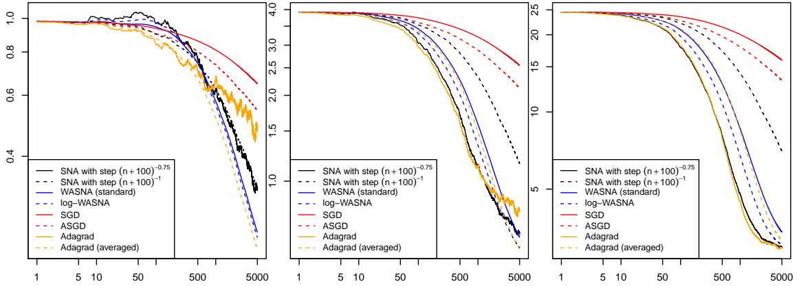
Figure 3: (Logistic regression with standard Gaussian variables) Mean-squared error of the distance to the optimum \theta with respect to the sample size for different initializations: \theta_0 = \theta + r_0 U , where U is a uniform random variable on the unit sphere of \mathbb{R}^d , with r_0 = 1 (left), r_0 = 2 (middle) or r_0 = 5 (right). Each curve is obtained by an average over 50 different samples (drawing a different initial point each time).
