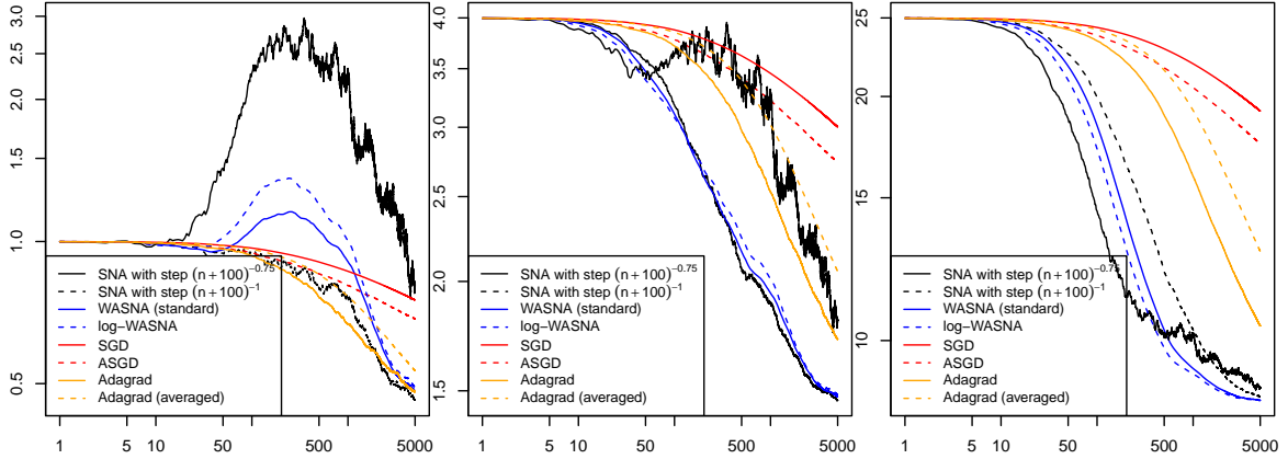
Figure 7: (Softmax regression with heteroscedastic Gaussian variables) Mean-squared error of the distance to the optimum \theta with respect to the sample size for different initializations: \theta_0 = \theta + r_0 U , where U is a uniform random variable on the unit sphere of \mathbb{R}^d , with r_0 = 1 (left), r_0 = 2 (middle) or r_0 = 5 (right). Each curve is obtained by an average over 50 different samples of size n = 5000 (drawing a different initial point each time).
