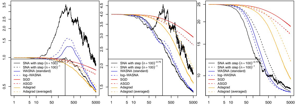
Figure 6: (Softmax regression with correlated Gaussian variables) Mean-squared error of the distance to the optimum \theta with respect to the sample size for different initializations: \theta_0 = \theta + r_0 U , where U is a uniform random variable on the unit sphere of \mathbb{R}^d , with r_0 = 1 (left), r_0 = 2 (middle) or r_0 = 5 (right). Each curve is obtained by an average over 50 different samples of size n = 5000 (drawing a different initial point each time).
