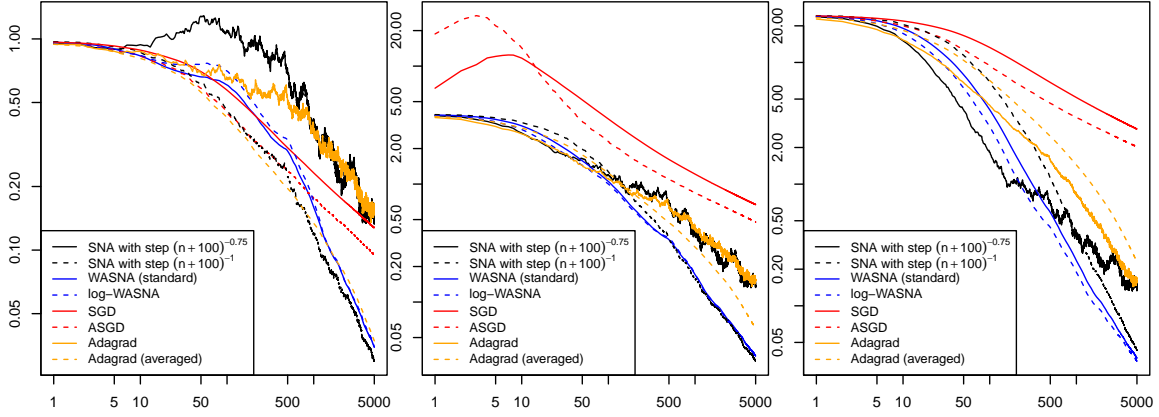
Figure 2: (Linear regression with correlated variables) Mean-squared error of the distance to the optimum \theta with respect to the sample size for different initializations: \theta_0 = \theta + r_0 U , where U is a uniform random variable on the unit sphere of \mathbb{R}^d , with r_0 = 1 (left), r_0 = 2 (middle) or r_0 = 5 (right). Each curve is obtained by an average over 50 different samples (drawing a different initial point each time).
