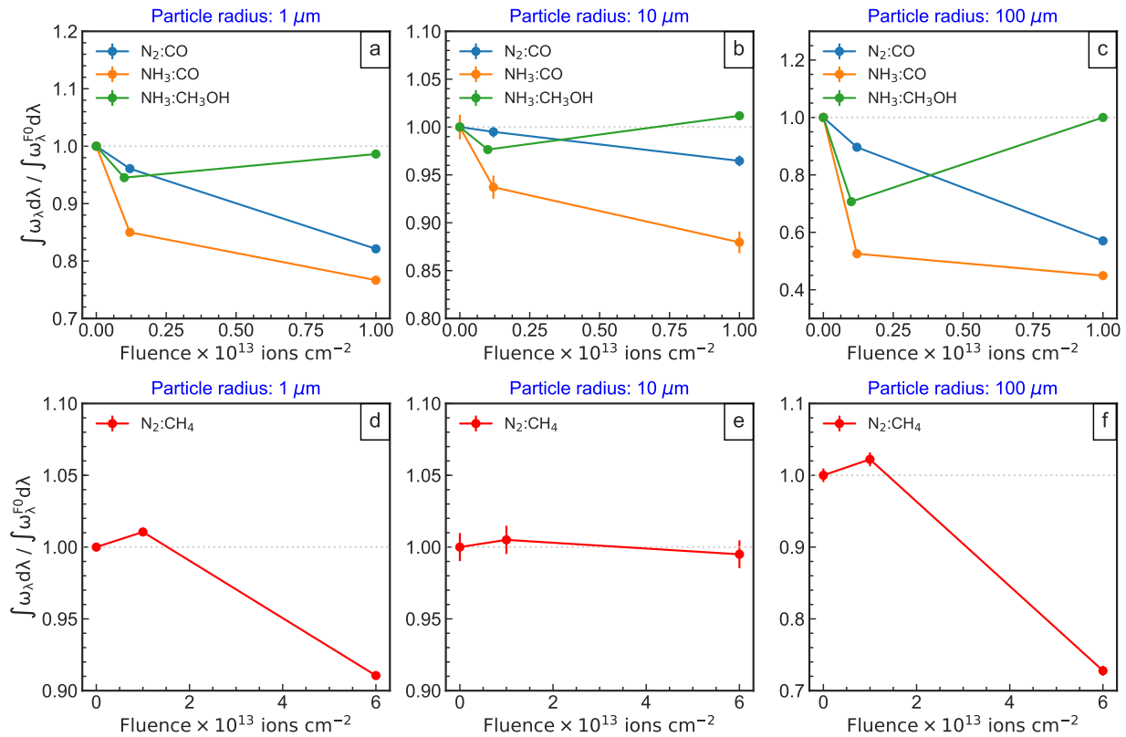
Figure 9: Same of Figure 8, but for the range between 2–5 \mu\text{m} .
