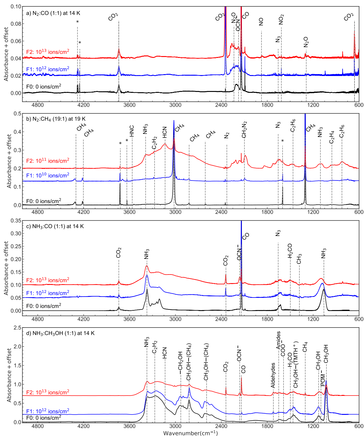
Figure 1: Absorbance infrared spectra of the four ice mixtures addressed in this paper. In order to assure a better readability, an arbitrary offset has been applied. The colours black, blue and red refer to the different fluences used in each experiment. Some vibrational modes associated to the bands are indicated by the vertical dashed grey line and their assignments is shown, as taken from [12, 24]. In the panel d , some bands are associated to different functional groups of molecules in literature, and are indicated by the chemical formula inside the parenthesis.
