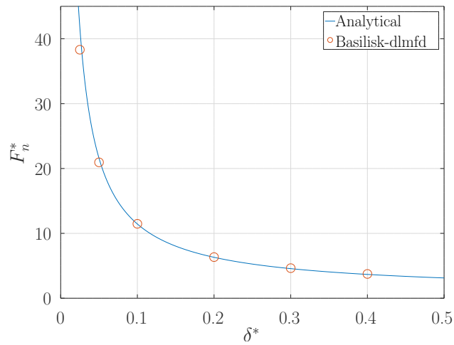
Figure 17: Comparison of our computed lubrication force for various gap distances against the analytical prediction of Brenner (1961) and Cooley and O'Neill (1969).
