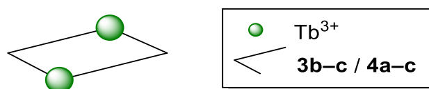
Figure 6. Schematic representation of the proposed structure for the 2:2 Tb(III)/ligand complexes formed with 3b–c and 4a–c .
