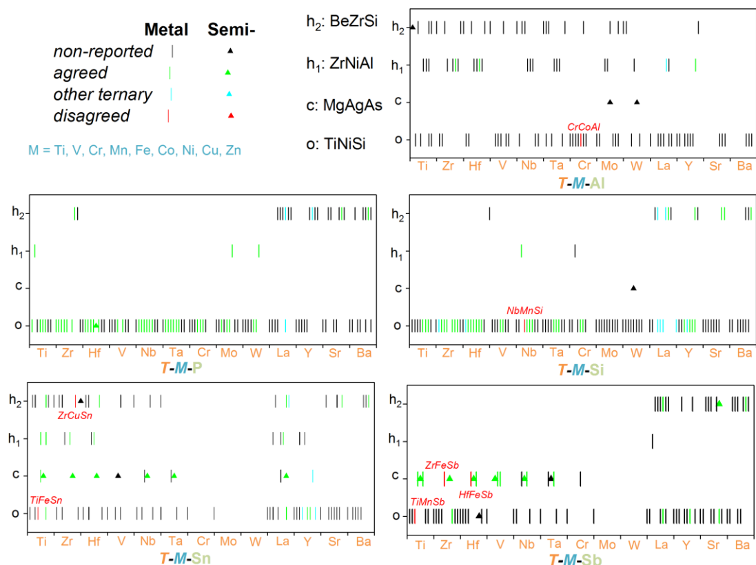
Figure 3: Plot of the calculated T-M-X configurations in their most stable structure-type; matching between calculated stable structure-type and reported data are defined by colour: black is for compounds which are not reported in the crystal databases, green represents the agreement, red is disagreement and blue is for compound reported in structure-type not included in our calculations. Vertical line corresponds to metallic compounds and triangle to semiconductors. For each T element, the 9 M elements are listed in the same order as in the periodic table (Ti, V, Cr ...).
