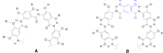
Figure 1. General structures of aromatic oligoamides having (A) an unsymmetrical (N-to-C) backbone and (B) a symmetrical backbone consisting of a central diacid residue (blue) and two identical groups. Hydrogen bonds are shown as dashed lines.
