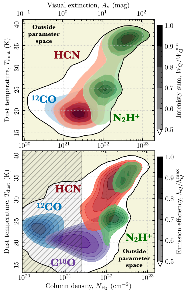
Figure 15. The total integrated intensity and emission efficiency [ h_Q = W(Q)/N_{H_2} ] as a function of column density and dust temperature for a selection of the molecular lines (see Figs 11 and 12). The contours show the 50, 60, 70, 80, and 90 per cent levels of total intensity in the upper panel, and emission efficiency in the lower panel. The black contour shows the region of the parameter space probed by the observations presented in this work. In the lower panel, we highlight values of the column density below N_{H_2}^{\text{thresh}} = 2.5 \times 10^{21} \text{ cm}^{-2} ( A_v^{\text{thresh}} = 2.7 mag) that suffer from increased ( > 30 per cent) uncertainties due to foreground and background contamination (see Section 3.1). Values of the h_Q below this threshold value should be taken with caution. This plot highlights the properties producing the most molecular line emission, and where the emission is being produced most efficiently.
