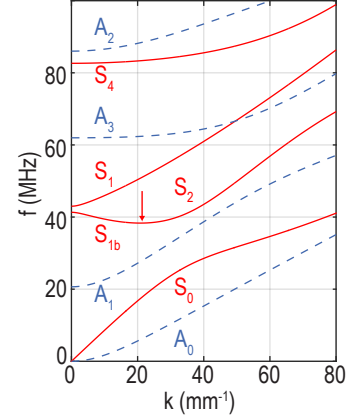
Figure 1: (Color online) Dispersion relations of Lamb waves for both symmetrical modes (solid red lines) and anti-symmetrical modes (dashed blue lines), the first ZGV mode is indicated by red arrow.
