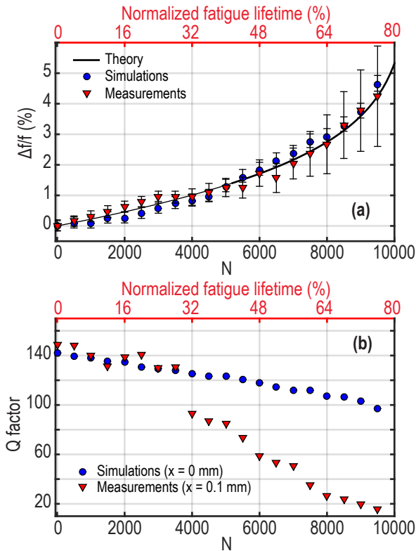
Figure 11: (a) Theoretical (solid line), experimental (triangles) and numerical evolution (circles) of the relative variation of the ZGV frequency at the center of the fatigued region as a function of the loading fatigue cycles N ; (b) Comparison of the experimental (triangles) and the numerical (circles) Q factors as a function of N .
