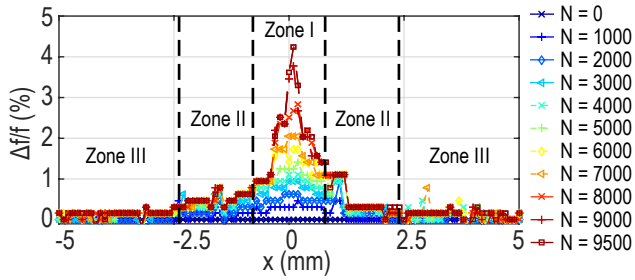
Figure 6: Experimental measurements of the spatial distribution of the ZGV resonance frequency for different fatigue cycles ( N = 0, 1000, 2000, \dots, 9000, 9500 ) and their qualitative classification in three regions.
