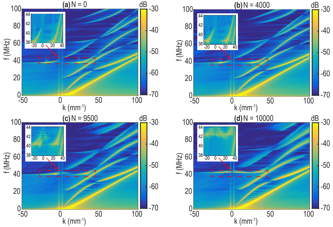
Figure 10: f - k diagram for the analyzes of the Lamb modes propagating in (a) an intact plate and (b-d) a damaged plate calculated from a set of 376 temporal signals with a spatial scanning step of 10 \mu\text{m} from x = 0 \text{ mm} to x = L_{\text{num}} = 3.75 \text{ mm} . Each temporal signal is calculated for a duration of 5 \mu\text{s} with a time step of 1 \text{ ns} .
