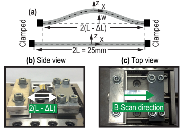
Figure 3: Fatigue configuration: (a) Illustration of the plate specimen loaded (top) and unloaded (bottom); (b) side-view photo of the loaded specimen; (c) top-view photo of the unloaded specimen.
