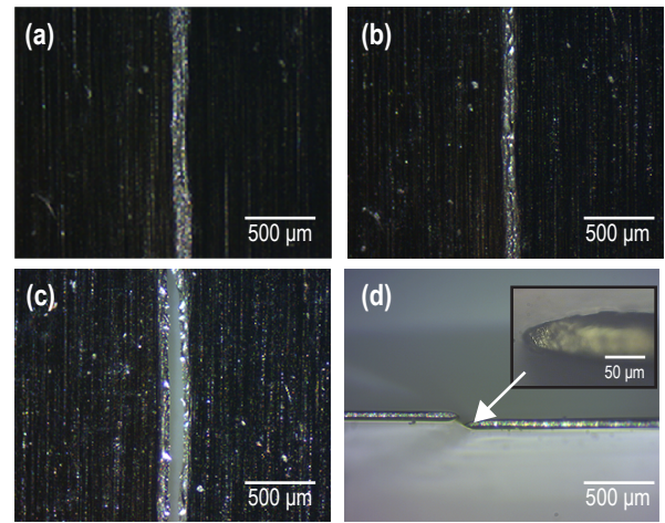
Figure 7: Top-view optical microscope photos of the fatigue progression on a specimen at (a) 30000 cycles, (b) 32000 cycles, and (c) \sim 33000 cycles (specimen failure). (d) Side-view of the broken specimen after 33000 cycles under optical microscope showing symmetrical decrease of the thickness around the fracture.
