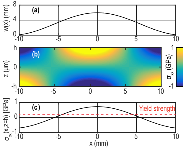
Figure 4: Buckling of a thin plate: (a) normal deflection of a plate with unloaded length of 2L = 25 mm and shortening length of 2\Delta L = 5 mm, (b) space distribution of the cross section stress \sigma_{xx} in (x, z) plane, and (c) surface stress distribution \sigma_{xx}(x, h) (solid line) and specimen's tensile yield strength (dashed red line)
