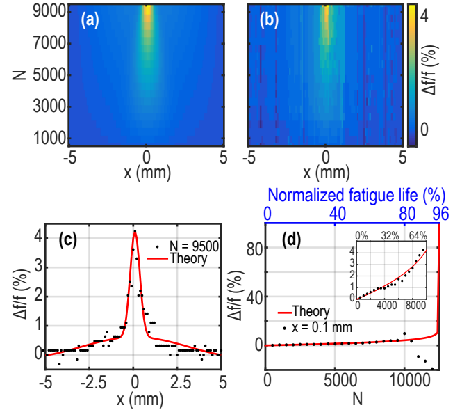
Figure 9: Comparison between theoretical model and experimental results: (a) distribution of theoretically calculated \Delta f/f as a function of the number of loading cycles N and of the lateral position x ; (b) distribution of experimental \Delta f/f as a function of the number of loading cycles N and of the lateral position x ; (c) comparison between experimental results and the theoretical fitting after 9500 fatigue cycles; (d) theoretical and experimental evolution of \Delta f/f in the center of the fatigued region (at x = \Delta x = 0.1 mm) as a function of the number of loading cycles N .
