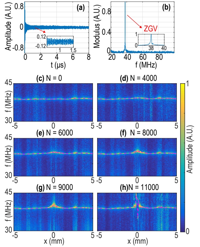
Figure 5: (a) Example of a received LU temporal signal on the intact specimen ( N = 0 ) and (b) its fast Fourier transform (FFT) with a sharp peak corresponding to the S_1S_2 -ZGV resonance frequency. Several chosen experimental measurements : amplitude spectrum density as a function of frequency ( f ) and specimen position ( x ) for loading cycles (c) N = 0 , (d) N = 4000 , (e) N = 6000 , (f) N = 8000 , (g) N = 9000 , and (h) N = 11000 .
