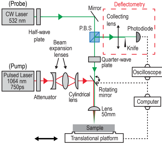
Figure 2: Experimental setup.
