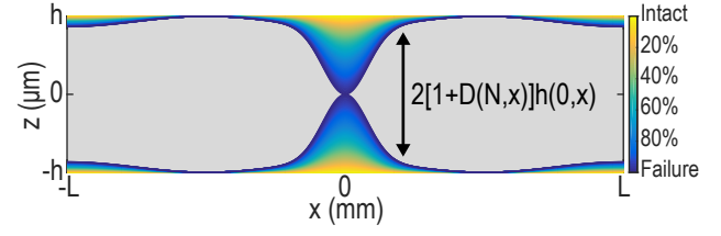
Figure 8: Illustration of the change in the specimen profiles caused by the fatigue damage. The gray background represents the remaining section of the plate after N_f fatigue cycles and the different color shades stand for the profile evolution of the plate subjected to fatigue damage: from the intact situation (light yellow) to the failure (dark blue) as indicated by the color bar. Numerical values of the input parameters for the calculation are: P_N = 50 , \sigma = 1 mm, \Delta x = 0 mm, 2L = 25 mm, \delta l = 0.1 mm, a_c = 0.98 , a_b = a_t = 0.01 , and the ratio N/N_f \in [0\%, 100\%] .
