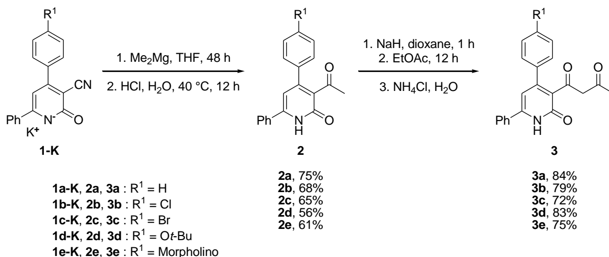
Scheme 2. Two-Step Synthesis of 1,3-Diketones 3 from 3-Cyano-2-pyridones 1-K.
