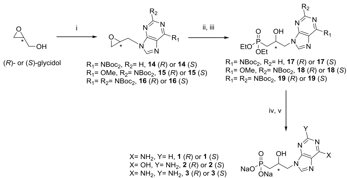
Scheme 2. Synthetic route to C3- \beta -hydroxy-ANPs containing adenine, guanine and 2,6-diaminopurine as nucleobases. Reagents & conditions: i) Bis(Boc)adenine, or bis(Boc)-2-amino-6- O -methylpurine, or tetra(Boc)-2,6-diaminopurine, \text{PPh}_3 , DEAD, THF, 0^\circ\text{C} to rt, 24 h; ii) Diethylphosphite, N,O -BSA, \text{CH}_2\text{Cl}_2 , reflux, 3-4 h; then addition of 14-16 in \text{CH}_2\text{Cl}_2 , -60^\circ\text{C} ; iii) \text{BF}_3 \cdot \text{Et}_2\text{O} , -60^\circ\text{C} to rt, overnight; iv) Trifluoroacetic acid in \text{CH}_2\text{Cl}_2 , 0^\circ\text{C} to rt, 5 h; v) \text{TMSBr} in \text{CH}_3\text{CN} , rt, 1-2 d, then \text{H}_2\text{O} , 0^\circ\text{C} to rt, 1 h.
