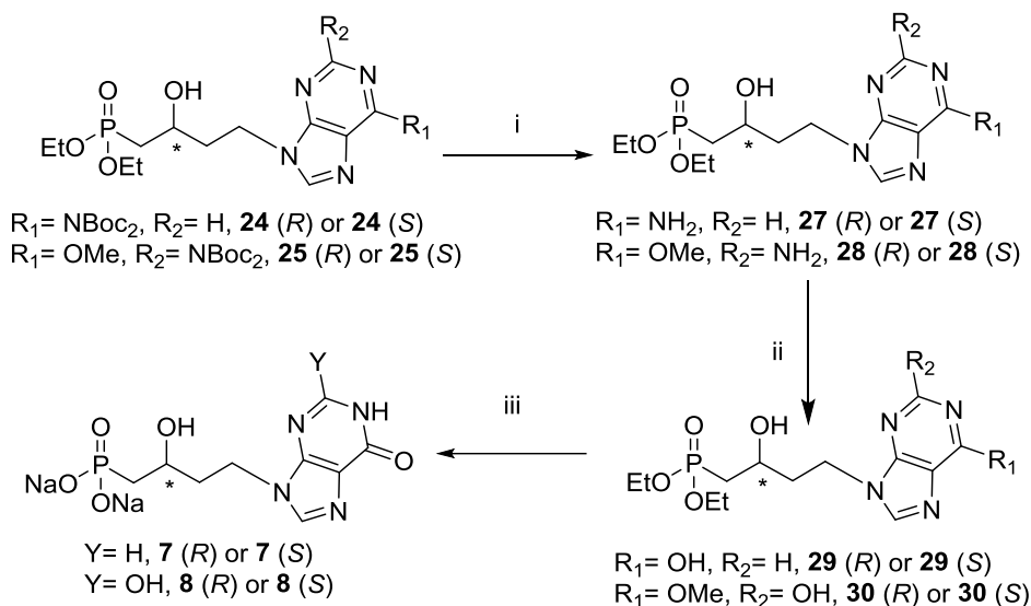
Scheme 4. Synthetic route to C4- \beta -hydroxy-ANPs containing xanthine and hypoxanthine as nucleobases. Reagents & conditions: i) Trifluoroacetic acid 20% in \text{CH}_2\text{Cl}_2 , 0^\circ\text{C} to rt, 45 min; ii) \text{NaNO}_2 , \text{H}_2\text{O} , \text{AcOH} 1M, 70^\circ\text{C} , 1 h; iii) \text{TMSBr} in \text{CH}_3\text{CN} , rt, 1-2 d, then TEAB, 0^\circ\text{C} to rt, 1 h.
