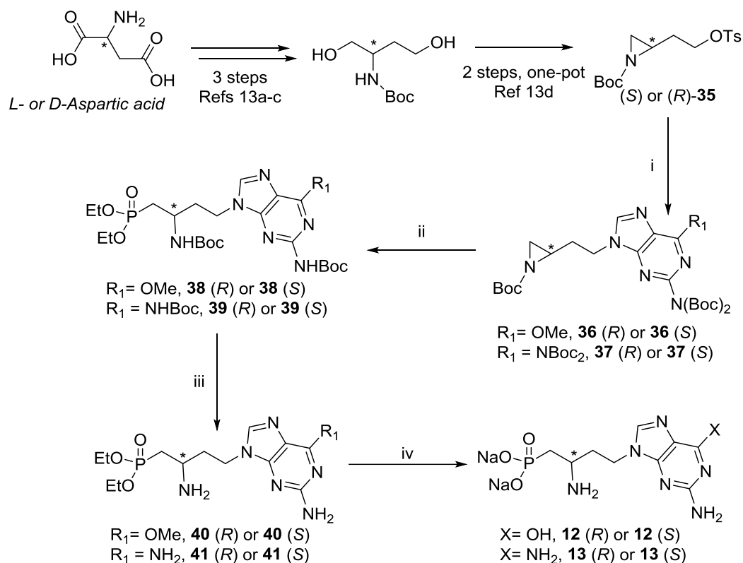
Scheme 6. Synthetic route to C4-β-amino-ANPs containing guanine and 2,6-diaminopurine as nucleobases. Reagents & conditions: i) Bis(Boc)-2-amino-6- O -methylpurine or tetra(Boc)-2,6-diaminopurine, K 2 CO 3 , DMF, rt, 3 d; ii) Diethylphosphite, LiHMDS, THF, -78°C, 15 min, then 36 or 37 was cannulated in THF, -78°C to rt; then rt overnight; iii) Trifluoroacetic acid in CH 2 Cl 2 , 0°C to rt, 5 h; iv) TMSBr in DMF, rt, 1-2 d, then TEAB, 0°C to rt, 1 h.
