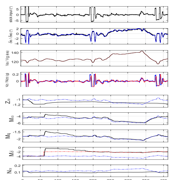
(b) FD estimation in varying flight conditions (altitude changes)
