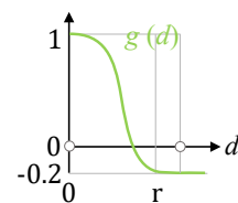
Fig. 8. Adaptability.
