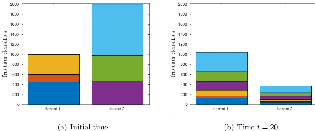
Figure 8: Evolution of I = 6 fractions in heterogeneous favorable environment: (a) 3 fractions (orange, red and blue) start in habitat 1 ( r_1 = 0.3 and K_1 = 1000 ) and 3 fractions start (light blue, green and purple) in habitat 2 ( r_2 = 0.01 and K_2 = 2000 ). The habitats are connected through asymmetric migration \varepsilon_{12} = 0.1 and \varepsilon_{21} = 0.3 . (b) distribution of the fractions in the two habitats at time t = 20 .
