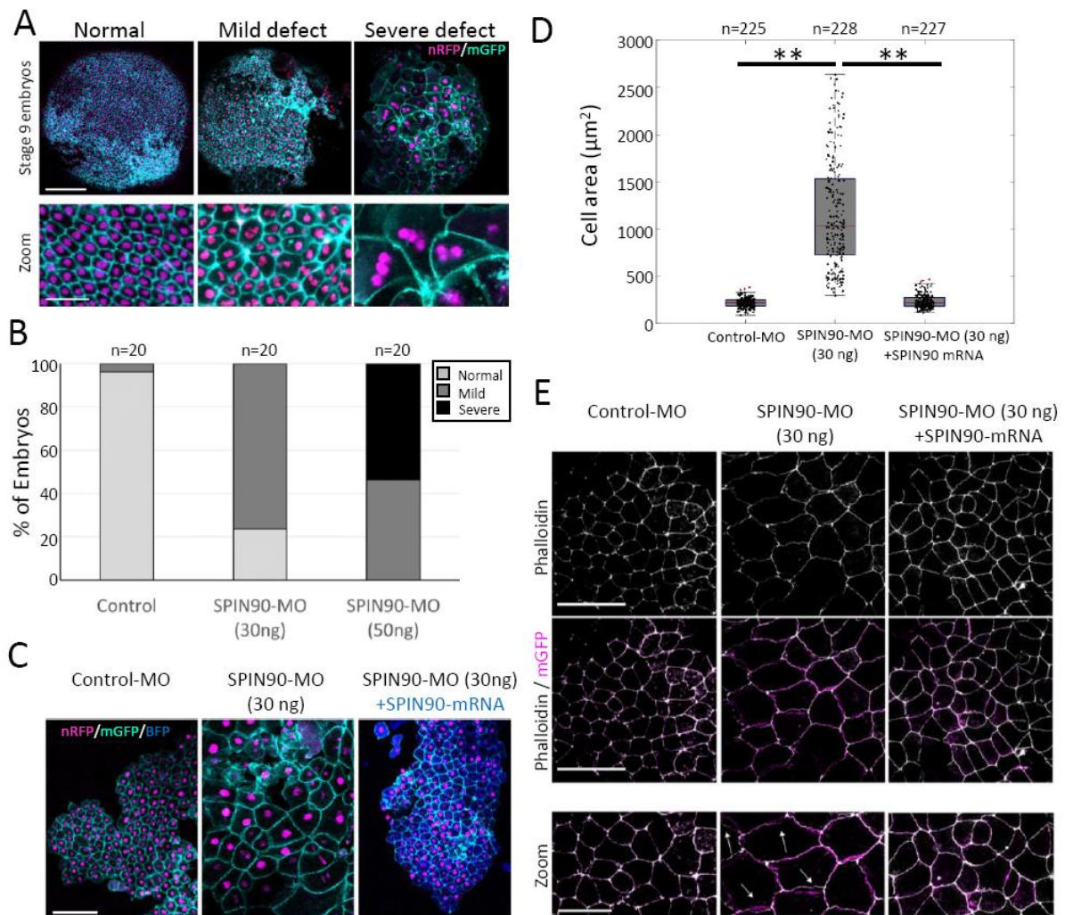
Figure 4. SPIN90 is necessary for correct development of Xenopus blastulae . A. Stage 9 Xenopus embryos (St9) injected with Control-MO or SPIN90-MO along with nuclear targeted RFP (nRFP) and membrane targeted GFP (mGFP). Images are representative of normal ectoderm (left) and ectoderm with mild (middle) or severe (right) defects in cell numbers and cell size. Scale bars: top row: 150 \mu\text{m} ; bottom row: 50 \mu\text{m} . B. Proportion of embryos with normal ectoderm (light grey) and mild (dark grey) or severe (black) defects for different morpholino injections. Experiments were repeated four times independently with similar results. Knock-down validation is presented in Supplementary Figure 5 . C. Stage 9 Xenopus embryos (St9) co-injected with: Control-MO (30ng), SPIN90-MO (30ng), or SPIN90-MO (30ng) plus full-length mouse SPIN90-BFP, along with nuclear targeted RFP and membrane targeted GFP. The efficiency of the rescue was 70% with just 10% of the embryos displaying morphant phenotype, compared to ~80% displayed by SPIN90-MO treated embryos. Images are representative of three independent experiments with similar results. Scale bar: 100 \mu\text{m} . D. Cell area for stage 9 Xenopus embryos injected with Control-MO (30ng), SPIN90-MO (30ng), or SPIN90 (30ng) + mouse SPIN90 mRNA. The distributions' medians, first and third quartiles and ranges are represented by the central red bars, bounding boxes and whiskers, respectively. The number of independent cellular measurements (n, indicated above each box) was pooled from three independent experiments. Statistical outliers are indicated by red dots. Statistical comparison with Welch's two-sided t-test: Control-MO vs SPIN90-MO: p=3 \times 10^{-131} ; SPIN90-MO vs rescue: p=5 \times 10^{-122} ; Control-MO vs rescue: p=0.20 . ** p < 0.01 . E. Stage 9 Xenopus embryos (St9) co-injected with Control-MO, SPIN90-MO, or SPIN90-MO plus full-length mouse SPIN90-BFP mRNA, along with membrane targeted GFP. Top panels display phalloidin staining (white), central panels show the overlap with membrane targeted GFP (magenta), and lower panels show a zoom of the middle panels. In some SPIN90-MO treated cells,
