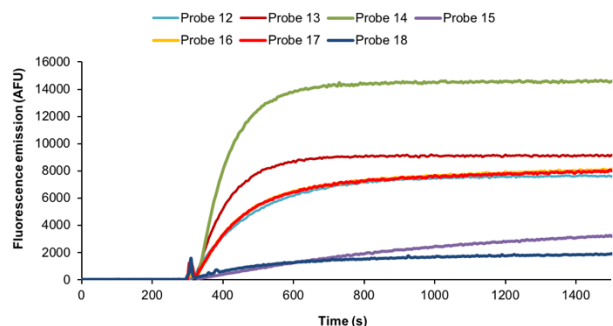
Figure 3. Time-dependent changes in the blue-green fluorescence intensity (Ex./Em. at the respective absorption/emission maxima, distinctive for each fluorophore, see the Supporting Information, slit = 2 nm) of fluorogenic probes 12–18 (concentration: 1.0 \mu M) in the presence of PGA (1 U) in PB (100 mM, pH 7.6) at 37 °C. Please note: PGA was added after 5 min of incubation of probe in PB alone.
