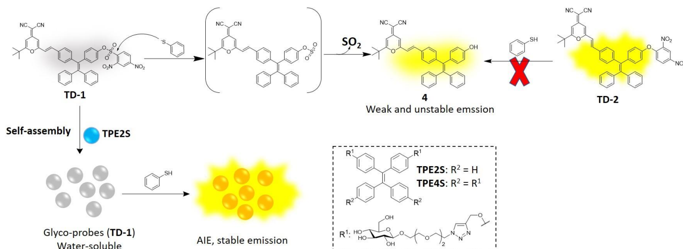
Scheme 1 TPE-DCM based fluorescent probe ( TD-1 ) and its glycol-probes self-assembled with TPE-based glycoclusters (TPE2S) for thiophenol (PhSH) detection.
