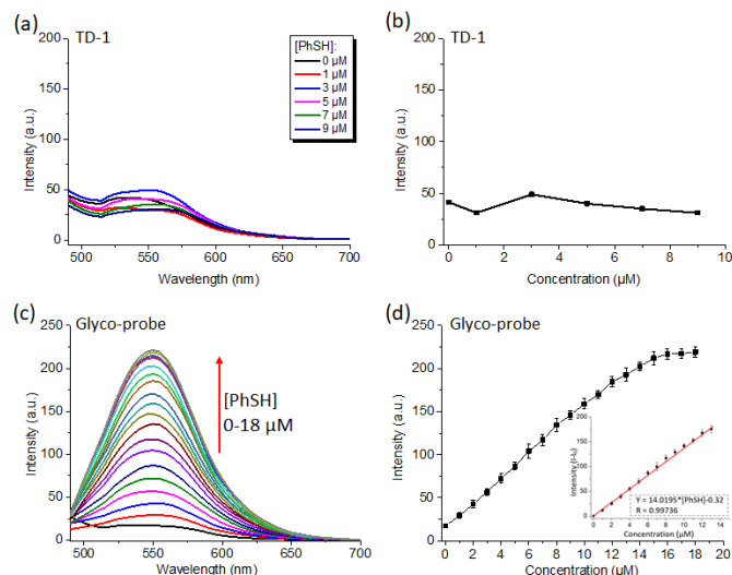
Figure 3 (a) and (b) Unstable fluorescence variation of TD-1 (10 \mu\text{M} ) response to thiophenol (0-9 \mu\text{M} ). (c) Fluorescence enhancement and (d) linear relationship of glyco-probe response to thiophenol (0-18 \mu\text{M} ) in 95% PBS buffer (pH 7.3, 10 mM) with THF during 5 min. ( \lambda_{\text{exc}} = 480 \text{ nm} )
