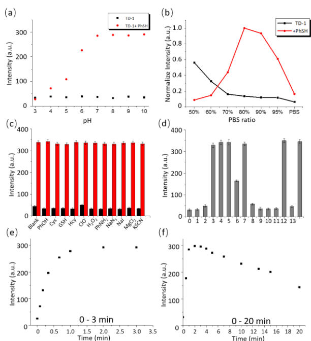
Figure 1 (a) Fluorescence variations of TD-1 (10 \mu M) before and after responding to thiophenol (100 \mu M) during 3 min in PBS buffer (pH 7.3) with 10% THF (pH was adjusted with HCl 0.6M or NaOH 2M). (b) ACQ and AIE effect influenced TD-1 response to thiophenol (100 \mu M) with addition of PBS buffer (pH 7.3) in THF during 10 min. (c) The fluorescence variation of TD-1 (10 \mu M) response to potential interfering species (50 \mu M) without (black bar) or with (red bar) thiophenol (100 \mu M) during 3 min. (d) TD-1 (10 \mu M) response to aliphatic and aromatic thiols (100 \mu M) during 3 min, Reagents: (0) Blank, (1) 1,2-ethanedithiol, (2) cyclohexanethiol, (3) m -NH 2 C 6 H 4 SH, (4) p -NH 2 C 6 H 4 SH, (5) p -MeOC 6 H 4 SH, (6) p -NO 2 C 6 H 4 SH, (7) p -MeC 6 H 4 SH, (8) 2-methyl-2-propanethiol, (9) pyrimidinethione, (10) \alpha -thioglycerol, (11) 2-mercaptobenzo-thiazole, (12) 4,4'-thiobisbenzenethiol, (13) 2-aminoethanethiol hydrochloride, (14) PhSH. (e) Fluorescence intensity increase of TD-1 (10 \mu M) incubating with thiophenol (100 \mu M) during 3 min. (f) Fluorescence intensity decrease of TD-1 (10 \mu M) incubating with thiophenol (100 \mu M) after 3-20 min due to probe separation from solution.
