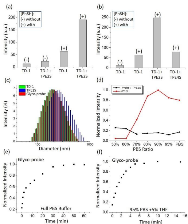
Figure 2 (a) Fluorescence changes of TD-1 (10 \mu\text{M} ) and glyco-probe after conjugation with TPE2S (10 mM) improved the fluorescence intensity for thiophenol (100 \mu\text{M} ) detection in 95% PBS (pH 7.3 10 mM) with THF. (b) Fluorescence enhancement abilities of TPE2S and TPE4S (10 mM) conjugating TD-1 (10 \mu\text{M} ) and detect thiophenol (100 \mu\text{M} ) in PBS buffer (pH 7.3, 10 mM). (c) DLS measurement of TD-1 , TPE2S and glyco-probe. (d) AIE effect influenced the glyco-probe response to thiophenol (100 \mu\text{M} ) with PBS buffer (pH 7.3, 10 mM) in THF during 5 min. (e) and (f) Response time of glyco-probe to thiophenol (100 \mu\text{M} ) in PBS buffer or PBS buffer with 5% THF.
