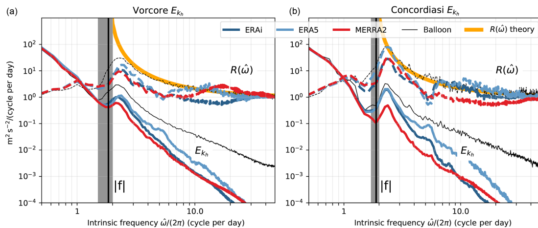
Figure 7. Intrinsic frequency spectra of horizontal kinetic energy per unit mass E_{kh} during the Vorcore (austral winter 2005; a ) and Concordiasi (austral winter 2010, b ) campaigns. The black curve corresponds to balloon observations during the campaigns, while the spectra estimated from isopycnic trajectories in different (re)analyses are in color. The vertical black line indicates the mean Coriolis parameter |f| , while the shaded gray area depicts its variability along the balloon trajectories.
