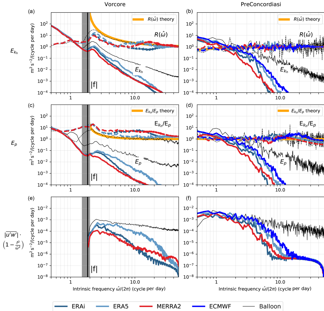
Figure 3. Intrinsic frequency spectra of (a, b) horizontal kinetic energy per unit mass E_{k_h} (solid) and rotary ratio R(\hat{\omega}) (dashed), (c, d) potential energy per unit mass E_p and ratio of kinetic over potential energy E_{k_h}/E_p , and (e, f) modules of the zonal pseudo-momentum flux per unit mass (1 - f^2/\hat{\omega}^2)|u'w'| during the polar Vorcore (a, c, e) campaign and the equatorial PreConcordiasi (b, d, f) campaign. The black curve on each plot corresponds to balloon observations, while the spectra estimated from isopycnic trajectories in different (re)analyses are in color. The vertical black line indicates the mean Coriolis parameter |f| , while the shaded gray area depicts its variability along the balloon trajectories. The trajectories used to compute the spectra are 8 d trajectories starting at the balloon position.
