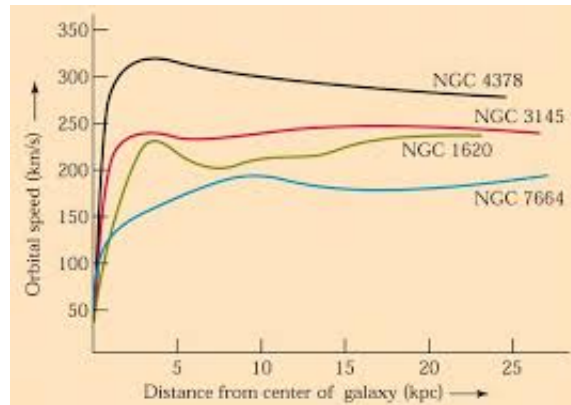
Figure 2: Some examples of rotation curves
