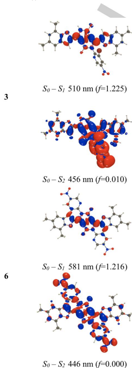
Figure 5. M06-2X density difference plots for the two lowest lying FC ES in dyes 3 and 6 . We recall that the vertical values have no exact experimental counterparts, but the trends in a homologous series are often restored. [29]
