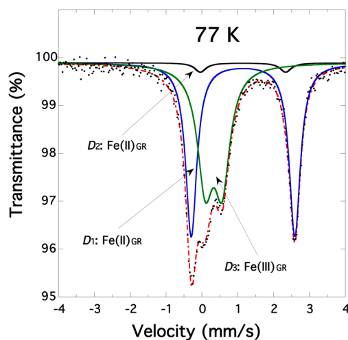
Figure 2. Transmission Mössbauer spectrum for biogenic hydroxycarbonate green rust recorded at 77 K. Experimental and fit curves are displayed as dotted black and dashed red lines, respectively. The fit components displayed as plain lines correspond to three doublets D_1 , D_2 and D_3 .
