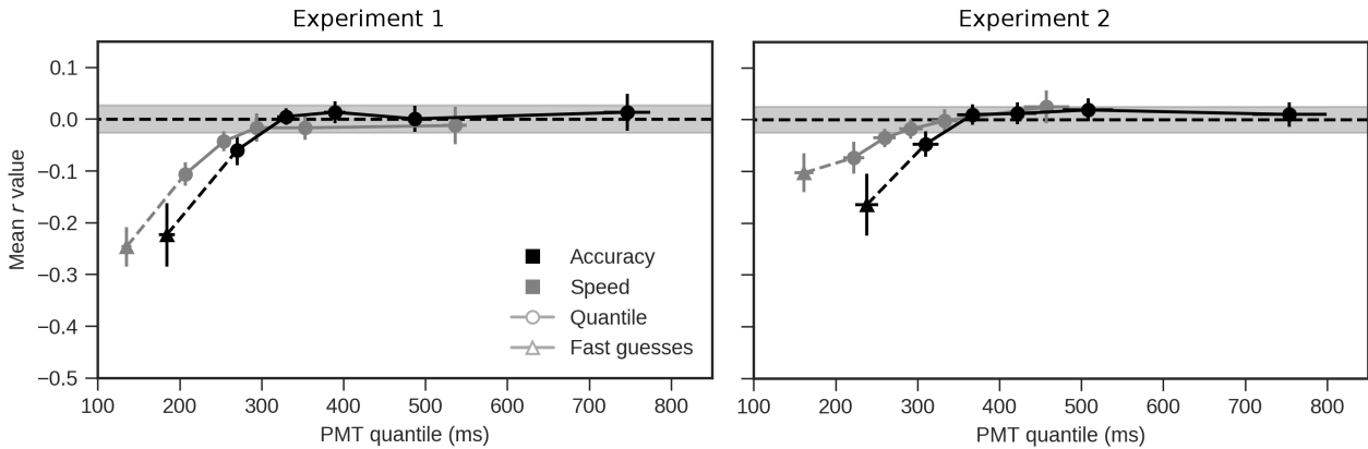
Figure 5. Mean Spearman correlations between PMT and MT for the trials identified as fast-guesses (triangles), and the PMT quantiles (circles) across both speed (gray) and accuracy (black) conditions for Experiment 1 (left) and Experiment 2 (right). Error bars represent one standard error of the mean. Shaded intervals represent 95 % confidence intervals of the correlation coefficient based on 1000 draws of the simulated random, normally distributed variables.
