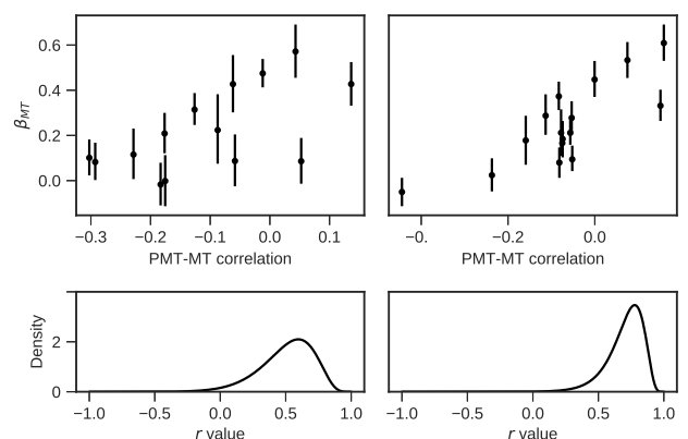
Figure 9. Representation of the correlation between the regression coefficient of MT over T_{er} plotted against the correlation between PMT and MT . Upper panels depicts scatterplots of both variables while lower panels represent plausible population correlation density for Experiment 1 (left panel) and Experiment 2 (right panel).
