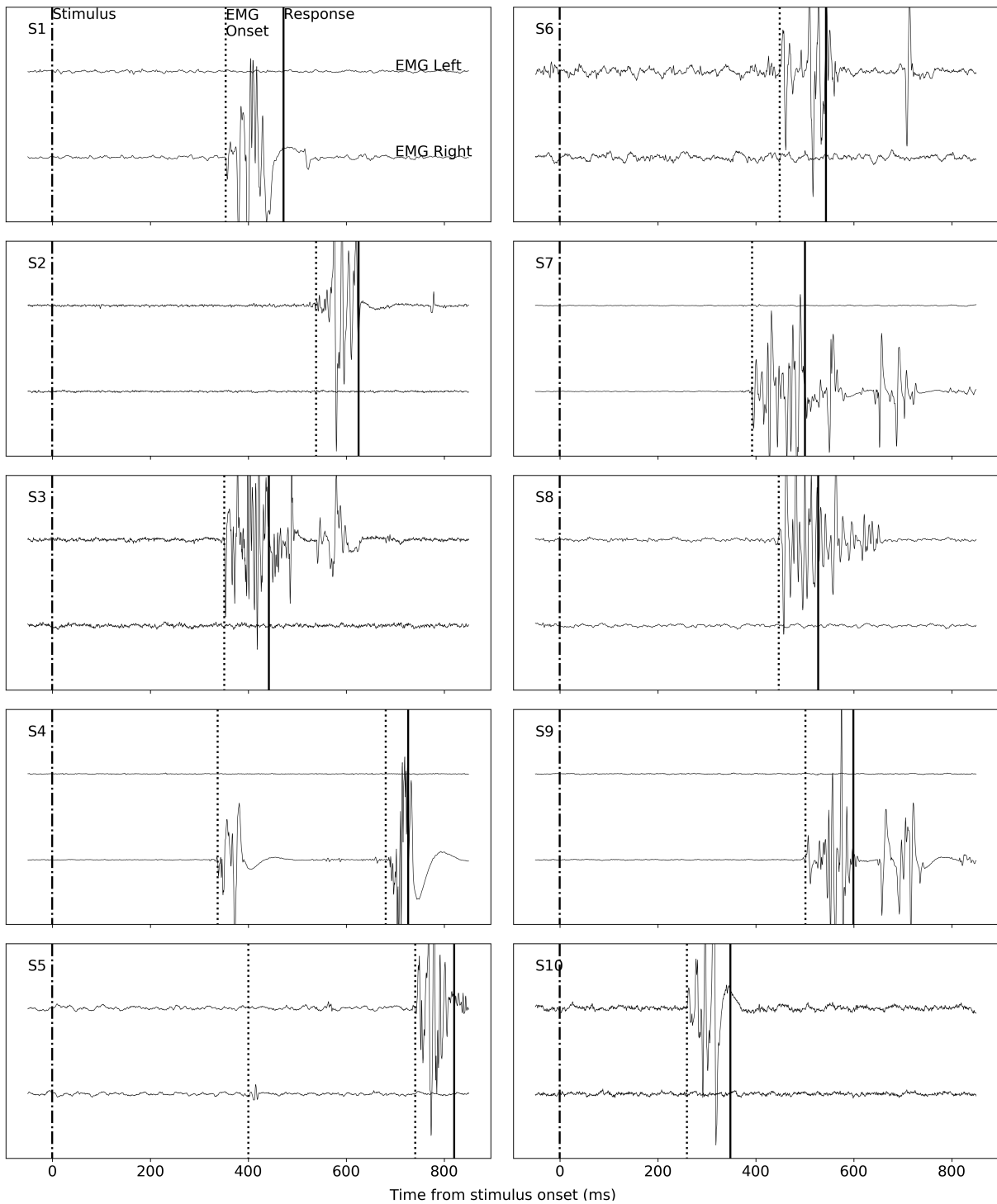
Figure A1. Graphic representation of the recorded EMG signal for the first trial of 10 participants in Experiment 1. Time is centered at stimulus onset (dot-dashed line), EMG onset(s) and recorded response are shown respectively with dotted line(s) and plain line. Left and right EMG signals are displayed respectively on the upper-and lower half of each panel. For graphical purpose values are z-scores of the amplitude (usually displayed in \mu V ), the data was read in Python using the MNE module (Gramfort et al., 2013).
