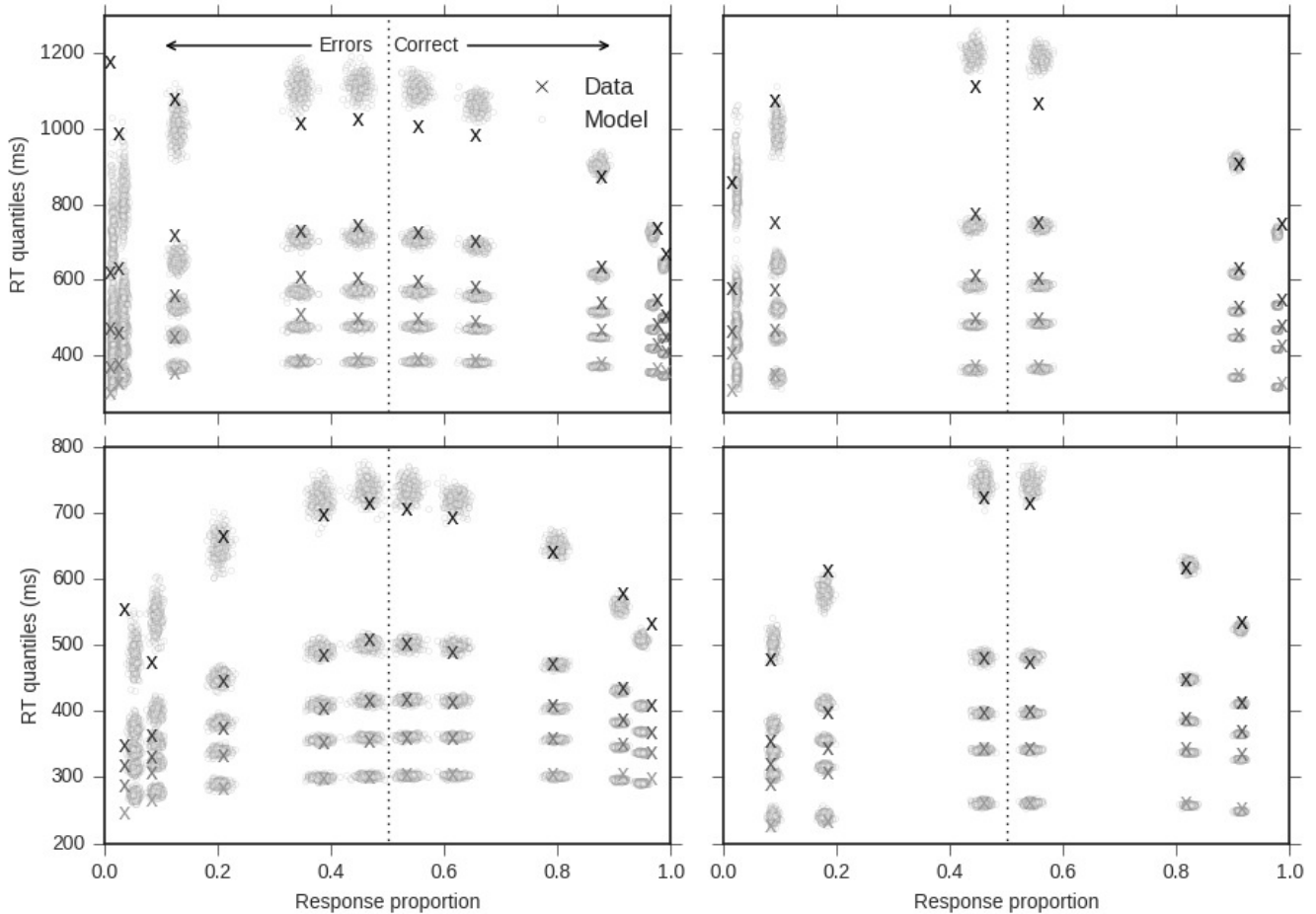
Figure 6. Quantile-probability plots (Ratcliff & McKoon, 2008) for Experiment 1 (left column) and Experiment 2 (right column), in the accuracy (upper row) and speed (lower row) conditions, computed from the winning model.
