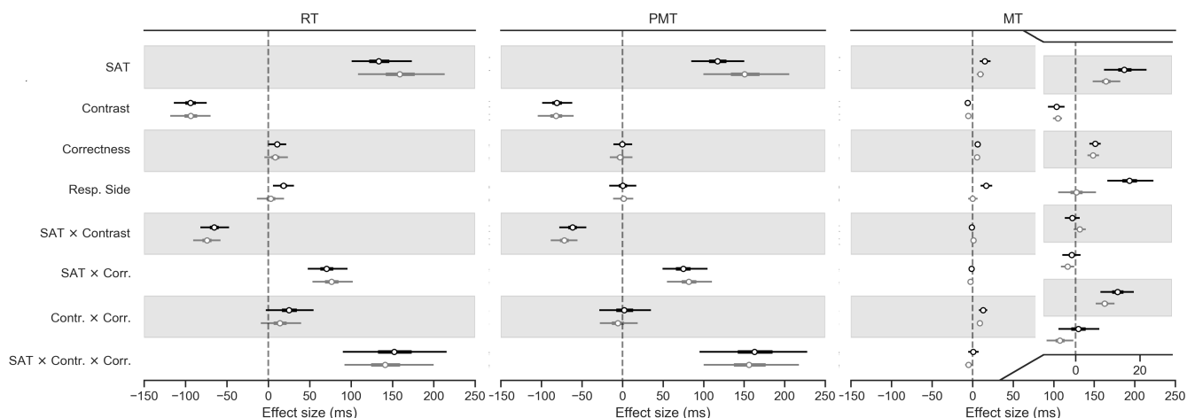
Figure 4. Posterior distributions for the regression coefficients from the LMM model fitted on the RT , PMT , and MT of Experiment 1 (black) and Experiment 2 (grey). The segments around the estimates represent 95% CrIs. As the coefficients for MT are of smaller magnitude, we provide a zoomed inset on the far right of the Figure to ease their visualisation.
