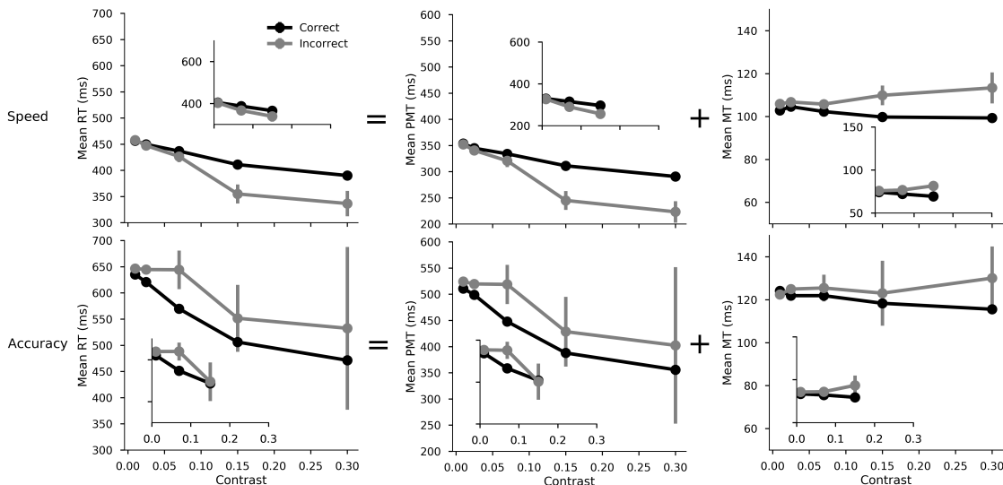
Figure 3. Observed results in Experiment 1, effect of stimulus strength level (contrast) on the mean RT (left column), PMT (center column) and MT (right column). This plot illustrates the interaction between contrast (x-axis), SAT conditions (top vs. bottom rows), and correctness of the response (black - correct vs. grey - incorrect). Bars around the mean represent 95% confidence intervals corrected for within-subject design using the method developed in Cousineau (2005). To assess replication, the small insets provide the results obtained in Experiment 2 for a subset of the contrast levels (0.01, 0.07, 0.15). Note: these figures analyze the means in millisecond units, while the LMM analysis presented in Table 1 model the means in log-transformed units.
