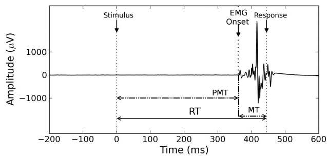
Figure 2. Single-trial RT decomposition using EMG. The Pre-Motor Time PMT is the time between stimulus and EMG onsets; the Motor Time MT is the time between the EMG onset and the mechanical response. See Figure A1 for additional examples of EMG recordings.
