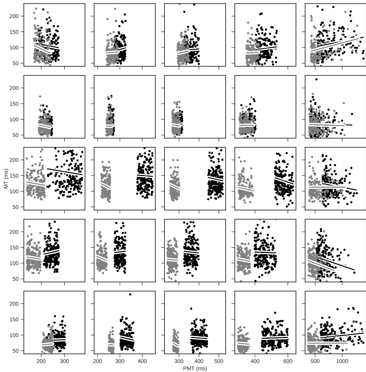
Figure D1. Scatter plots of PMT versus MT for the 5 first participants in Experiment 1 (participant 1 to 5 from top to bottom) across the 5 quantiles (.1, .3, .5, .7 and .9 quantiles, from left to right) either with the speed (gray) or accuracy (black) instructions. In order to give a sense of the linear relationship between the pairs of PMT and MT , each scatter plot is associated with a line drawn from the parameters of a linear regression of MT over PMT , estimated using the ordinary least squares method as implemented in the statsmodel python package (Seabold & Perktold, 2010).
