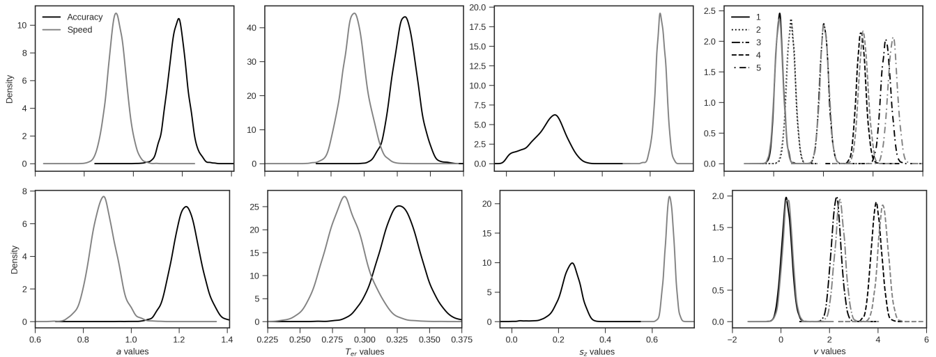
Figure 7. Posterior distributions of the parameters left free to vary across conditions. Top row is for Experiment 1, bottom row for Experiment 2. a , T_{er} , s_z , v stand for boundary separation, non-decision time, inter-trial variability of the starting point and drift rate. For the drift rate (last panel), numbers in the legend represent contrast levels.
