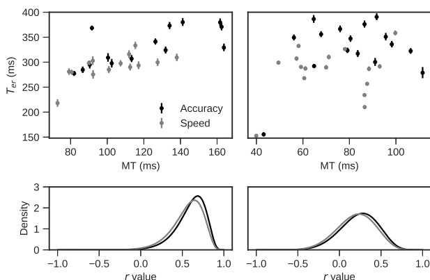
Figure 8. Correlation between the estimated T_{er} and the measured MT , computed by participant. Upper row: scatterplots of the MT and T_{er} pairs for each participant; lower row: plausible population correlation density. Left column: Experiment 1; right column: Experiment 2.
