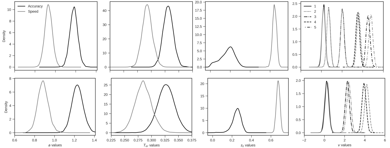
Figure 7. Posterior distributions of the parameters left free to vary across conditions.
