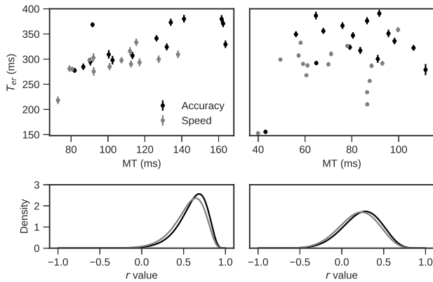
Figure 8. Correlation between the estimated T_{er} and the measured MT , computed by participant.
