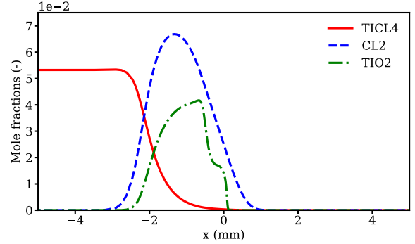
(b) Titania species mole fractions.
