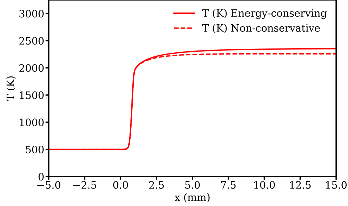
Figure 3 – Comparison of the temperature profiles obtained with the energy-conserving model and the non-energy-conserving one. Same conditions as in Figures 1.
