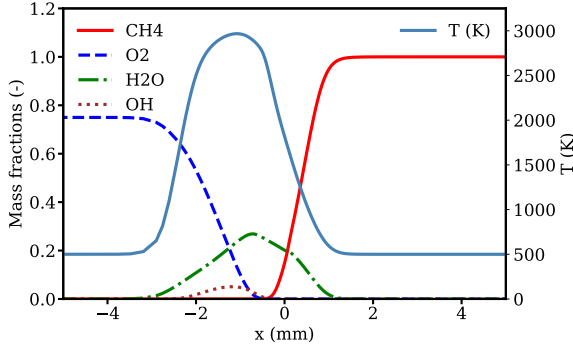
(a) Main species mass fractions and temperature.
