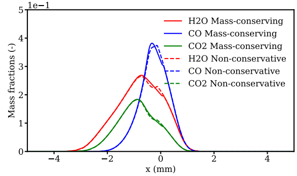
(b) Mass fraction profiles of \text{H}_2\text{O} , \text{CO} and \text{CO}_2 .
