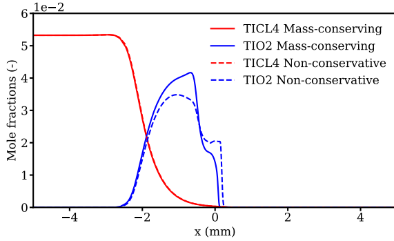
(a) \text{TiCl}_4 and \text{TiO}_2 mole fraction profiles.
