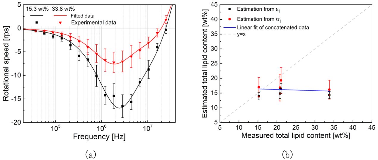
Figure 10. (a) The fitting of experimental electrorotation spectra of S. abundans containing 15.3 wt% and 33.8 wt% of lipids by using the double-shell ellipsoidal model with constant cell wall thickness; (b) The relationship between measured total lipid contents and calculated lipid contents from permittivities ( \epsilon_I ) and conductivities ( \sigma_I ) of inner core shown in table 4.
