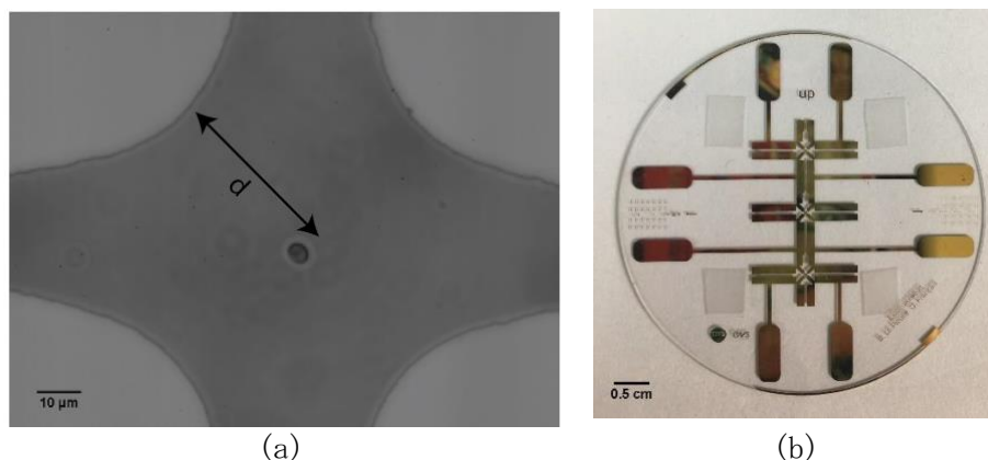
Figure 1. Device for conducting electrorotation of single microalgae cells: (a) single microalgae cell ( S. abundans ) captured at the center of the microelectrode set; (b) the device overview.
