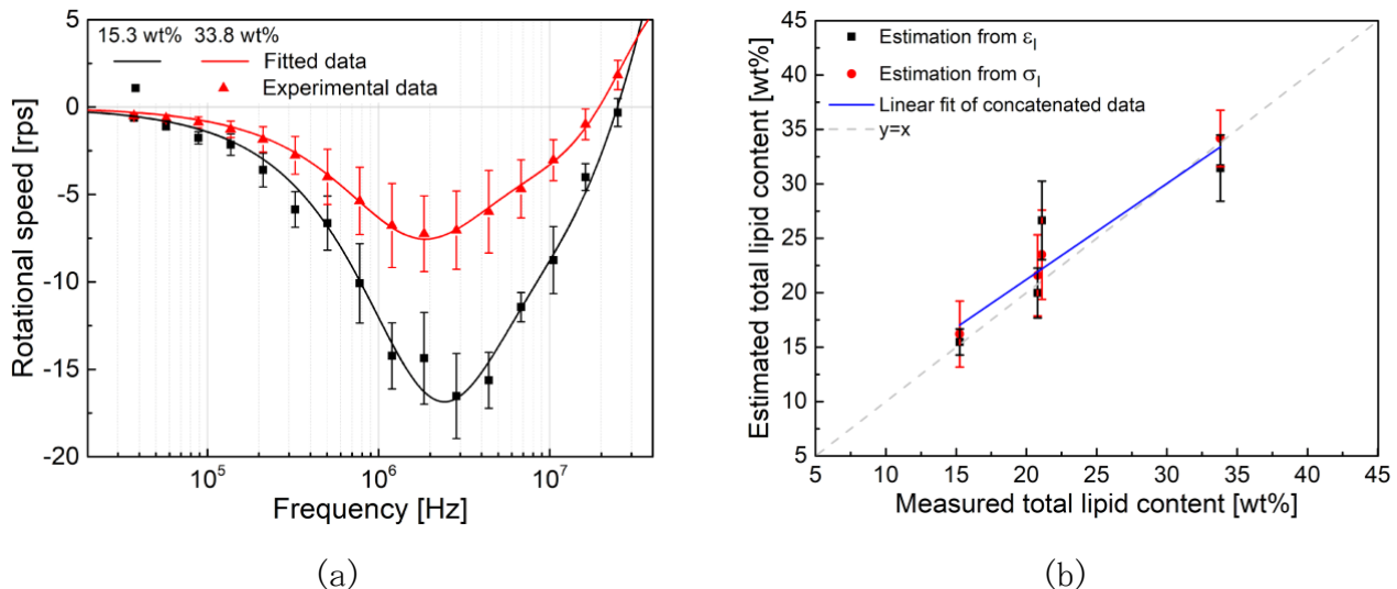
Figure 9. (a) The fitting of experimental electrorotation spectra of S. abundans containing 15.3 wt% and 33.8 wt% of lipids by using the double-shell ellipsoidal model considering cell wall; (b) The relationship between measured total lipid contents and calculated lipid contents from permittivities ( \epsilon_I ) and conductivities ( \sigma_I ) of inner core listed in table 3.
