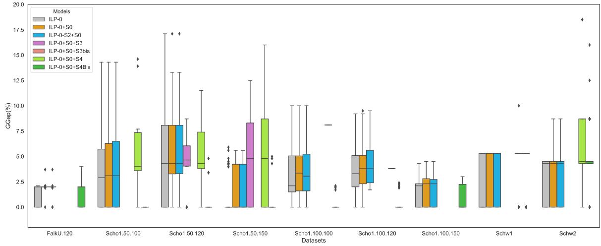
Fig. 6: Comparison of the gurobi gaps (%) of formulations ILP-0 , ILP-0+S0 , ILP-0-S2+S0 and ILP-0+S0+Si for i in \{3, 3Bis, 4, 4Bis\} on the data-sets from BPPLIB, when disabling Gurobi Optimizer proprietary cuts
