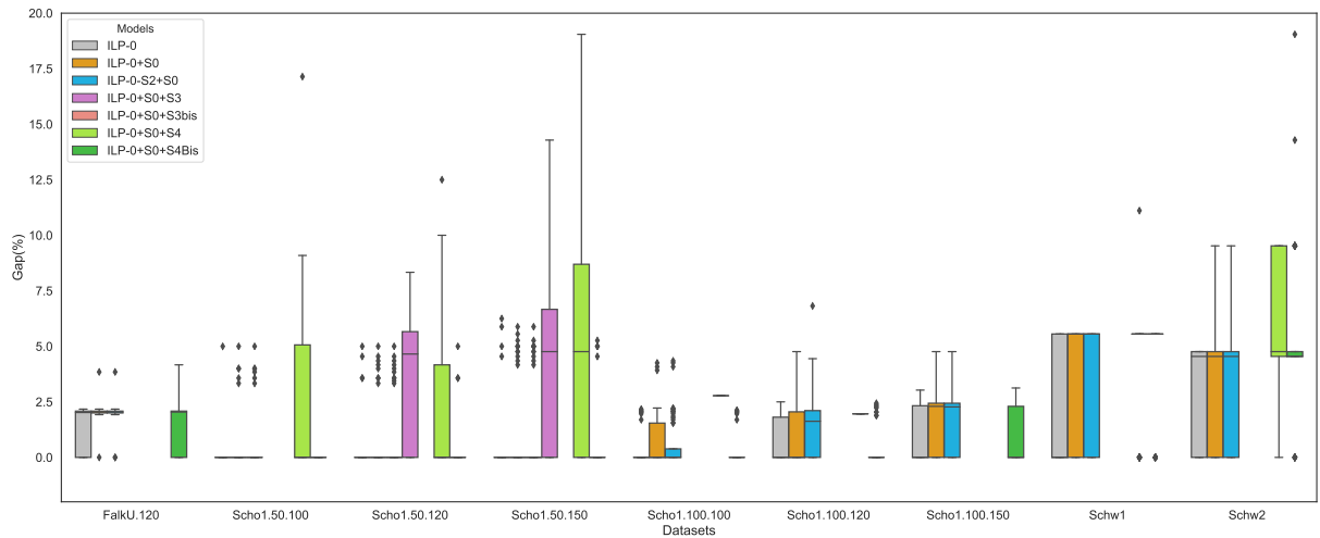
Fig. 7: Comparison of the gaps (%) of formulations ILP-0 , ILP-0+S0 , ILP-0-S2+S0 and ILP-0+S0+Si for i in \{3, 3Bis, 4, 4Bis\} on the data-sets from BPPLIB, when disabling Gurobi Optimizer proprietary cuts
