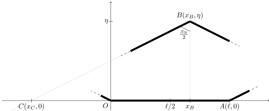
Figure 10: An N -gon with all angles equal to \beta_N .
