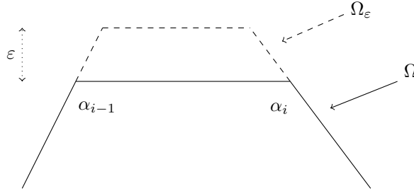
Figure 9: Parallel displacement of one side.
