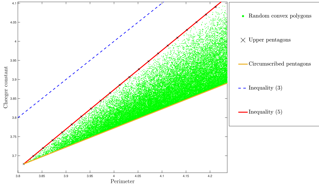
Figure 11: Blaschke-Santaló diagram of convex pentagons.
