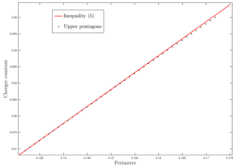
Figure 12: A zoom on the upper boundary.
