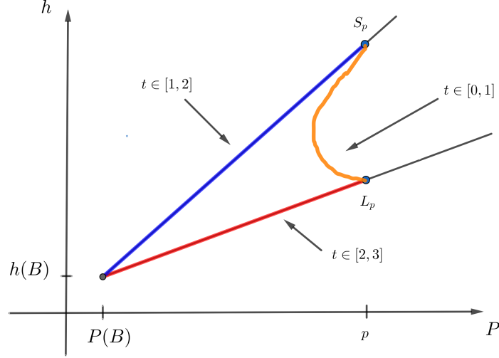
Figure 5: The continuous and closed path \Gamma_p .
