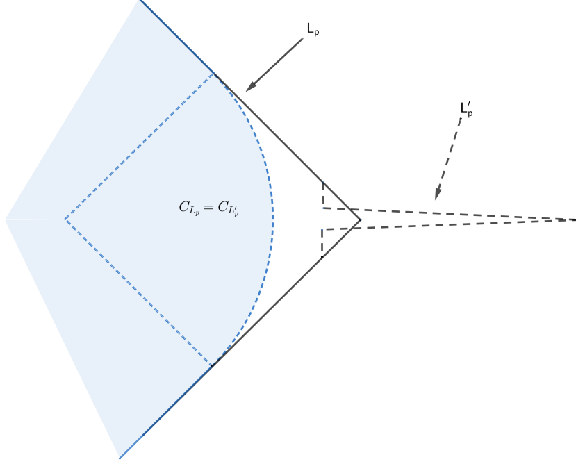
Figure 6: Tailed domain L'_p with the same area and Cheeger set and higher perimeter.
