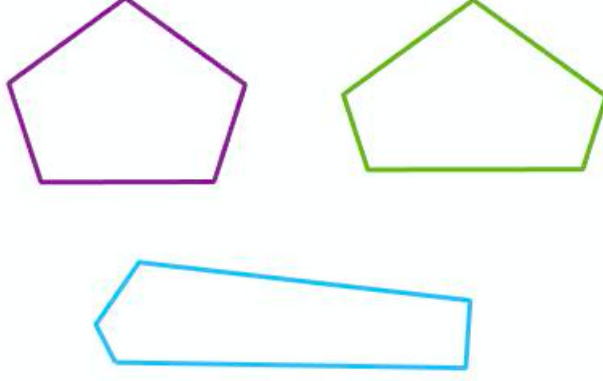
Figure 13: Optimal pentagons obtained for p_0 \in \{3.86, 4, 5\} .
