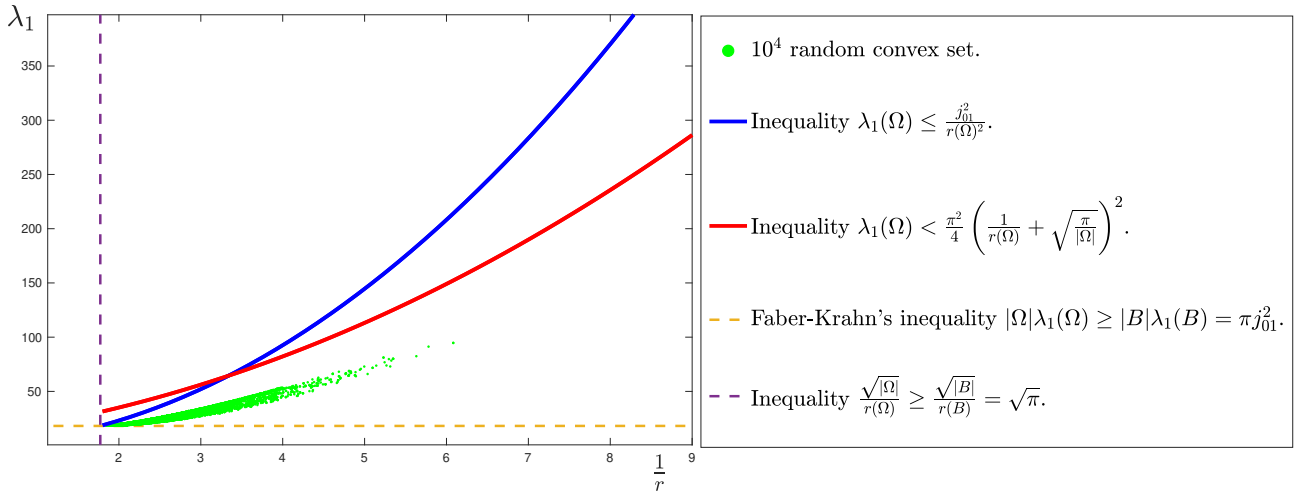
Figure 5: Inequality (8) improves (11) for convex sets with small inradius (ie. large \frac{1}{r} ).
