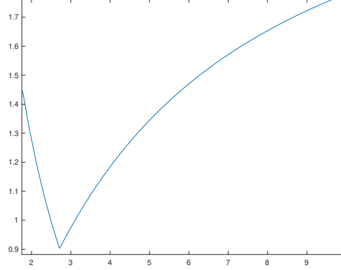
Figure 3: Curve of the function x \mapsto \frac{\max(\pi j_{01}^2, \frac{\pi^2 x^2}{4})}{(x + \sqrt{\pi})^2} .
