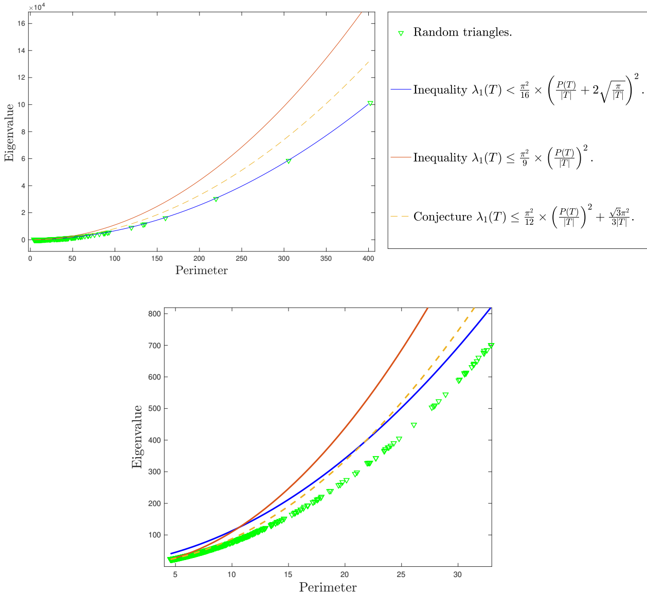
Figure 6: Comparison between inequalities (12) and (13) and Conjecture (14) with a zoom on smaller values of the perimeter.
