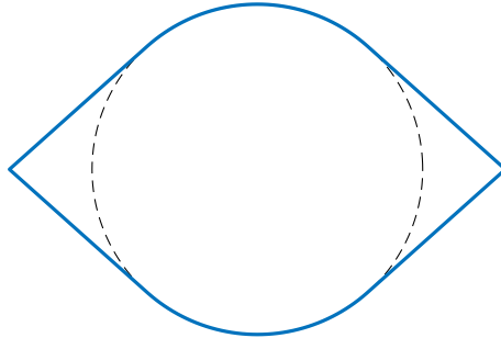
Figure 2: A symmetrical 2-cap body.
