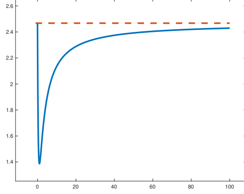
Figure 4: The curve of \Psi_{(0,1)} .
