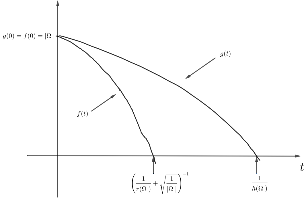
Figure 3: Idea of proof of the upper bound.
