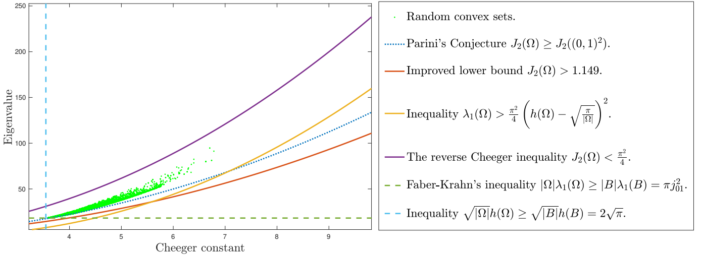
Figure 7: Approximation of the Blaschke-Santaló diagram \mathcal{C} and relevant inequalities.
