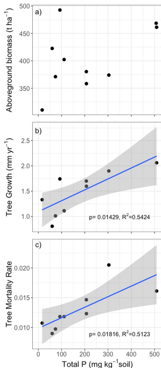
Figure 6. (a) Aboveground biomass ( \text{t ha}^{-1} ), (b) tree growth rate ( \text{mm yr}^{-1} ) for trees >10 cm diameter, and (c) tree mortality rates for trees >10 cm diameter from nine 1 ha forest plots across French Guiana plotted against soil total phosphorus concentrations in the top 0–15 cm of the soil. Blue lines are linear model fits and grey areas are 95% confidence intervals. In (a) there is no significant fit ( p = 0.1676 ) so no fit is shown. One extra site is included in (a) because one year of aboveground biomass data was available, however multi-year dynamic growth and mortality rates were not available.
