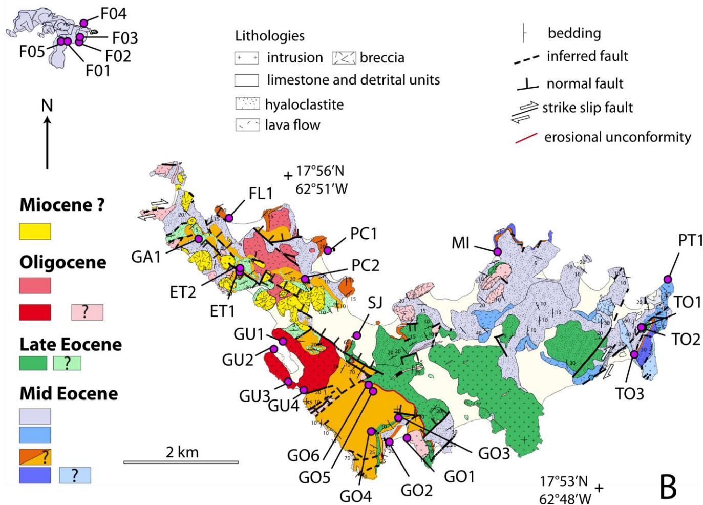
(caption on next page) Fig. 1. A) Structural map of the northeastern Caribbean plate. Di-erent blocks are mapped (from Byrne et al., 1985; Stein et al., 1988; Calais et al., 2010; Symithe et al., 2015) and are separated by the main crustal scale structures a-ecting the upper plate (from Mann et al., 1995, 2005; Grindlay et al., 2005; Roux, 2007; Feuillet et al., 2002, 2011; Legendre et al., 2018; Laurencin, 2017; Laurencin et al., 2018; De Min, 2014; Leroy et al., 2015). Other lineaments are drawn from the GEBCO (Guidelines for the General Bathymetric
