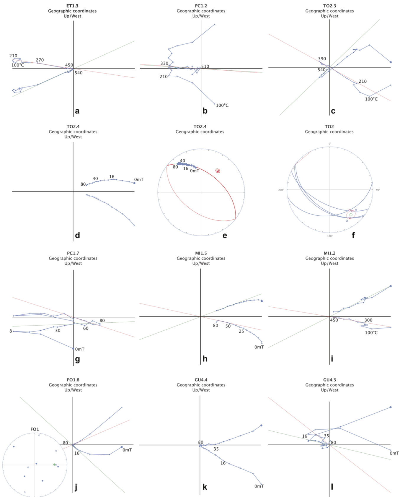
Fig. 2. Representative Zijdeveld diagrams and great circle plots of the sampled lithologies of St. Barthélemy and Île Fourchue. See text for further details.
