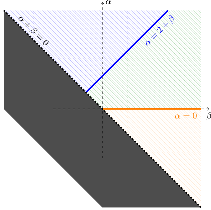
FIGURE 2. Presentation of the results in the (\alpha, \beta) plane. Admissible parameters are in half-plane \alpha + \beta > 0 . The blue hatched area leads to \theta(\varepsilon) = \varepsilon^2 and a standard diffusive limit with symbol \kappa|\xi|^2 . The blue line is the set of parameters yielding the anomalous scaling \theta(\varepsilon) = \varepsilon^2 |\ln(\varepsilon)| but still a standard diffusive limit with symbol \kappa|\xi|^2 . The green hatched area results into the fractional scaling \theta(\varepsilon) = \varepsilon^{\frac{\alpha+\beta}{1+\beta}} and a fractional diffusive limit with symbol \kappa|\xi|^{\frac{\alpha+\beta}{1+\beta}} . The orange bold line yields the fractional scaling \theta(\varepsilon) = \varepsilon^{\frac{\beta}{1+\beta}} |\ln(\varepsilon)| and a fractional diffusive limit with symbol \kappa|\xi|^{\frac{\beta}{1+\beta}} . Finally, the orange hatched area yields the fractional scaling \theta(\varepsilon) = \varepsilon^{\frac{\beta}{1+\beta}} and a fractional diffusive limit with symbol \kappa|\xi|^{\frac{\beta}{1+\beta}} .
