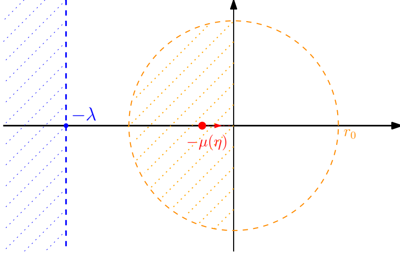
FIGURE 1. The blue dashed zone on the left of \text{Re} z = -\lambda corresponds to the spectral gap estimates on \tilde{L}^* + i\eta|v|^\beta(v \cdot \sigma) due to the coercivity Hypothesis 2. The orange dashed zone is where Lemmas 1.1-1.2 construct a unique real eigenvalue -\mu(\eta) \sim -\mu_0\Theta(\eta) of the latter operator, that goes to zero as \eta \rightarrow 0 .
