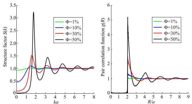
FIG. 1. (Color online) Example of structure factor S(k) and corresponding pair correlation function g(R) for an isotropic distribution of impenetrable spheres with identical radius a for several volume fractions \Phi = 1\% , 10%, 30%, and 50%.
