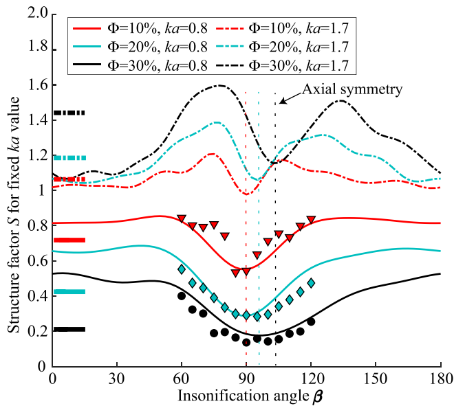
FIG. 7. (Color online) Structure factor at fixed value of ka as a function of the insonification angle \beta for volume fractions \Phi = 10\% , 20\% , and 30\% . The thin solid and dashed lines represent the structure factors obtained from the Stokesian dynamics numerical simulations for ka = 0.8 and ka = 1.7 , respectively. The thick solid and dashed lines on the left side represent the theoretical BSC_{theo} computed by the SFM in the isotropic case for ka = 0.8 and ka = 1.7 , respectively. The symbols represent the structure factors measured by ultrasound S_{meas}(ka = 0.8) .
