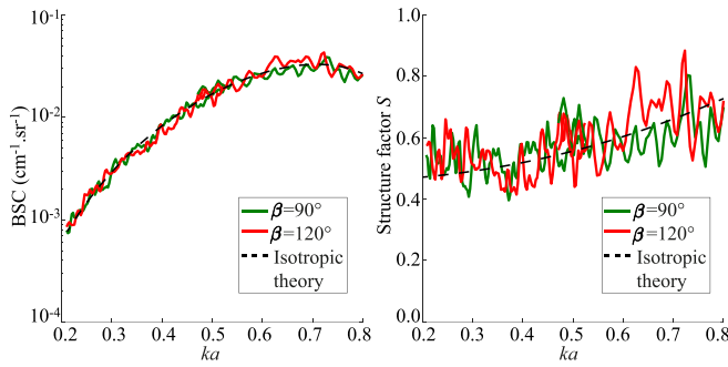
FIG. 3. (Color online) Measured BSC_{meas} and corresponding structure factors S_{meas} (solid lines) from a suspension mixed by hand ( \Phi = 10\% ). Measurements were performed for two insonification angles \beta = 90^\circ and 120^\circ .
