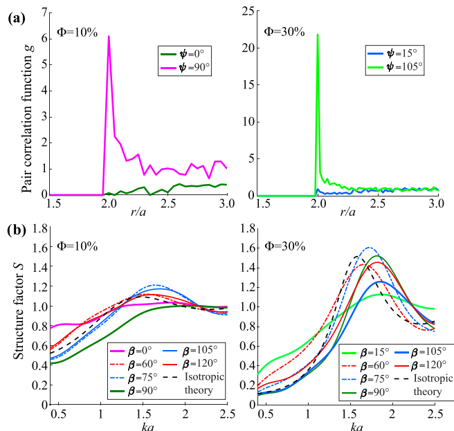
FIG. 6. (Color online) (a) 1D scalar plots of the numerical pair correlation function g for volume fractions \Phi=10\% and 30\% . (b) Numerical structure factors S at various insonification angles \beta for volume fractions \Phi=10\% and 30\% .
