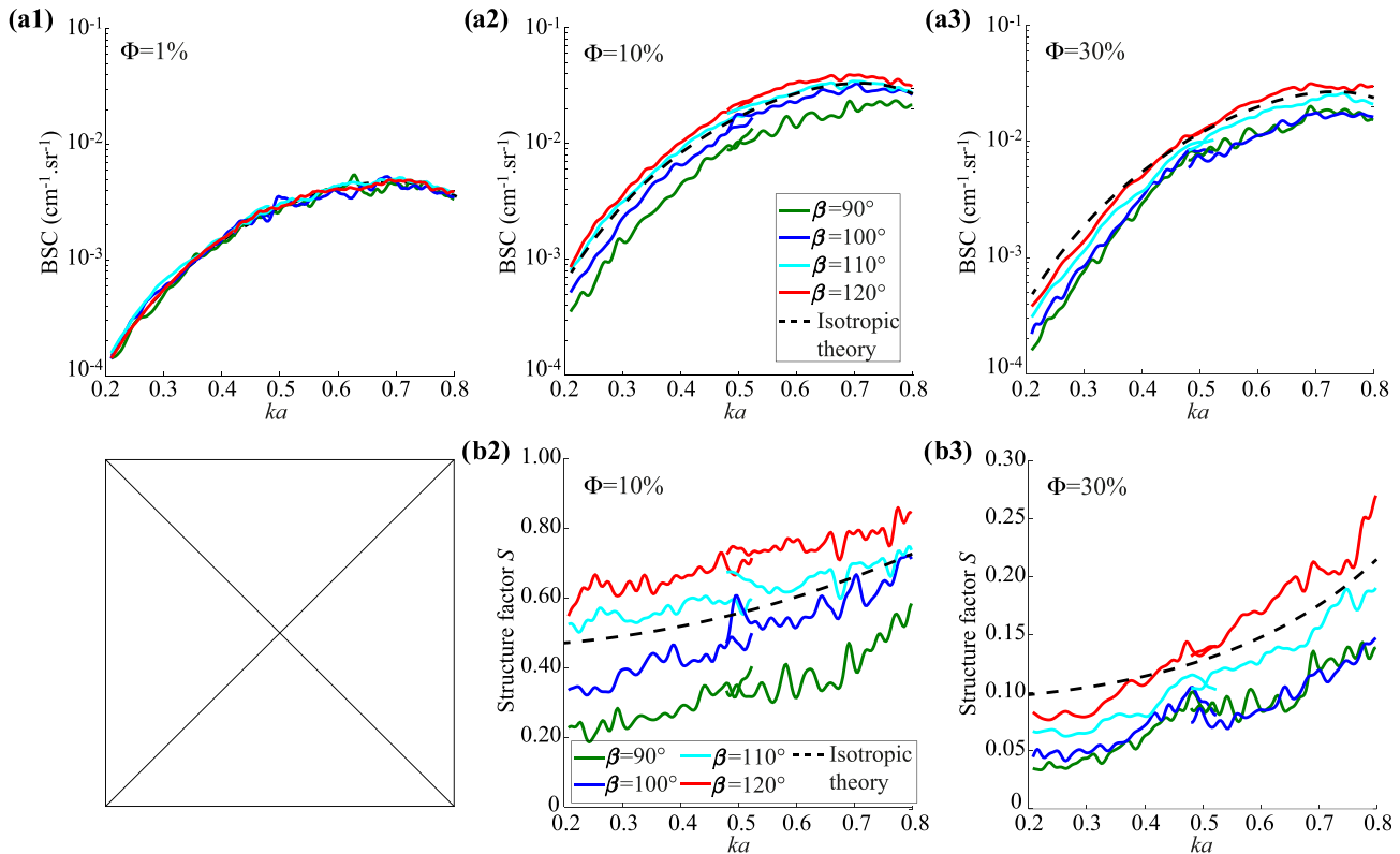
FIG. 4. (Color online) (a) Measured BSC_{meas} as a function of the product ka (solid lines) from suspensions sheared in the Couette device at various insonification angles \beta for volume fractions \Phi = 1\% , 10%, and 30%. Also represented are the theoretical BSC_{theo} computed by the SFM in the isotropic case (dashed lines). (b) Same as (a) for the structure factor as a function of the product ka . Note that the structure factor at \Phi = 1\% is not represented because it cannot be computed for the lowest volume fraction of 1%.
