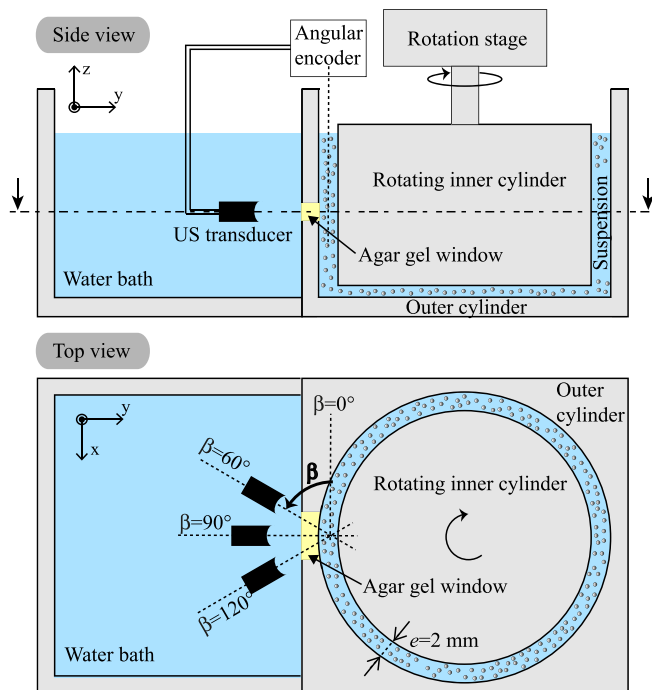
FIG. 2. (Color online) Schematic of the setup, top and side view.
