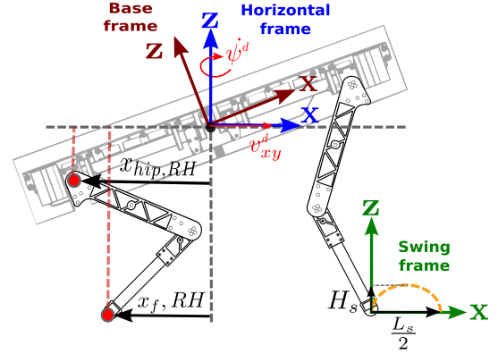
Fig. 6: Frames used by the foothold planner. Desired base twist and foothold positions are expressed in the horizontal frame. Each step is taken with respect to a "virtual foothold" that moves with the base and represents the nominal size of the stance of the gait cycle (e.g. when the desired twist is set to zero)
