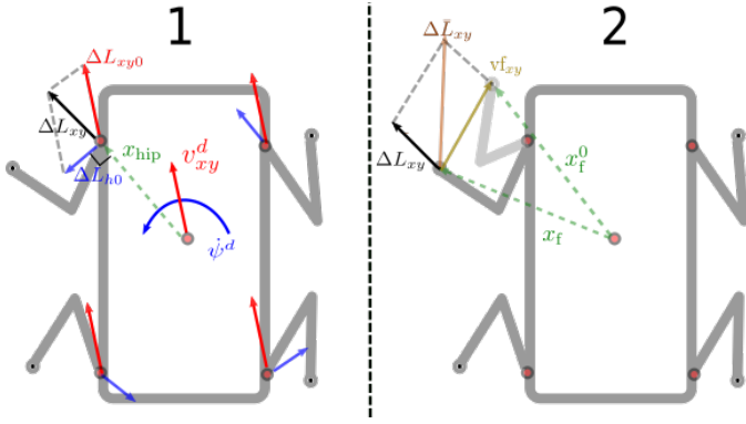
Fig. 7: Top view of the robot with the geometrical explanation of the foot displacements computation: 1) starting from the desired linear \mathbf{v}_{xy}^d and angular \psi^d velocities, we compute the corresponding deltas \Delta \mathbf{L}_{xy0} and \Delta \mathbf{L}_{h0} . 2) The resulting vector \Delta \mathbf{L}_{xy} is then summed to the virtual foothold vector \mathbf{v}_{f_{xy}} to produce the total foot displacement \Delta \bar{\mathbf{L}}_{xy} .
