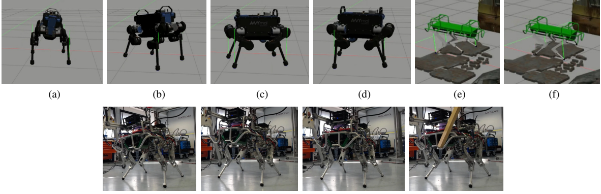
Fig. 8: First row: snapshots of the locomotion simulations: ANYmal tracking a (a) roll reference, a (b) pitch reference, (c),(d) changing the robot height. HyQ during a (e) crawl swinging only one leg at a time and a trot (f) swinging two legs at the time. Second row: snapshots of the trunk orientation experiments with HyQ. The robot is tracking an orientation reference while being disturbed by an external interaction.
