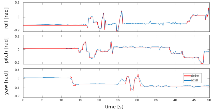
Fig. 10: Real hardware - HyQ changing the base orientation in roll, pitch and yaw.
