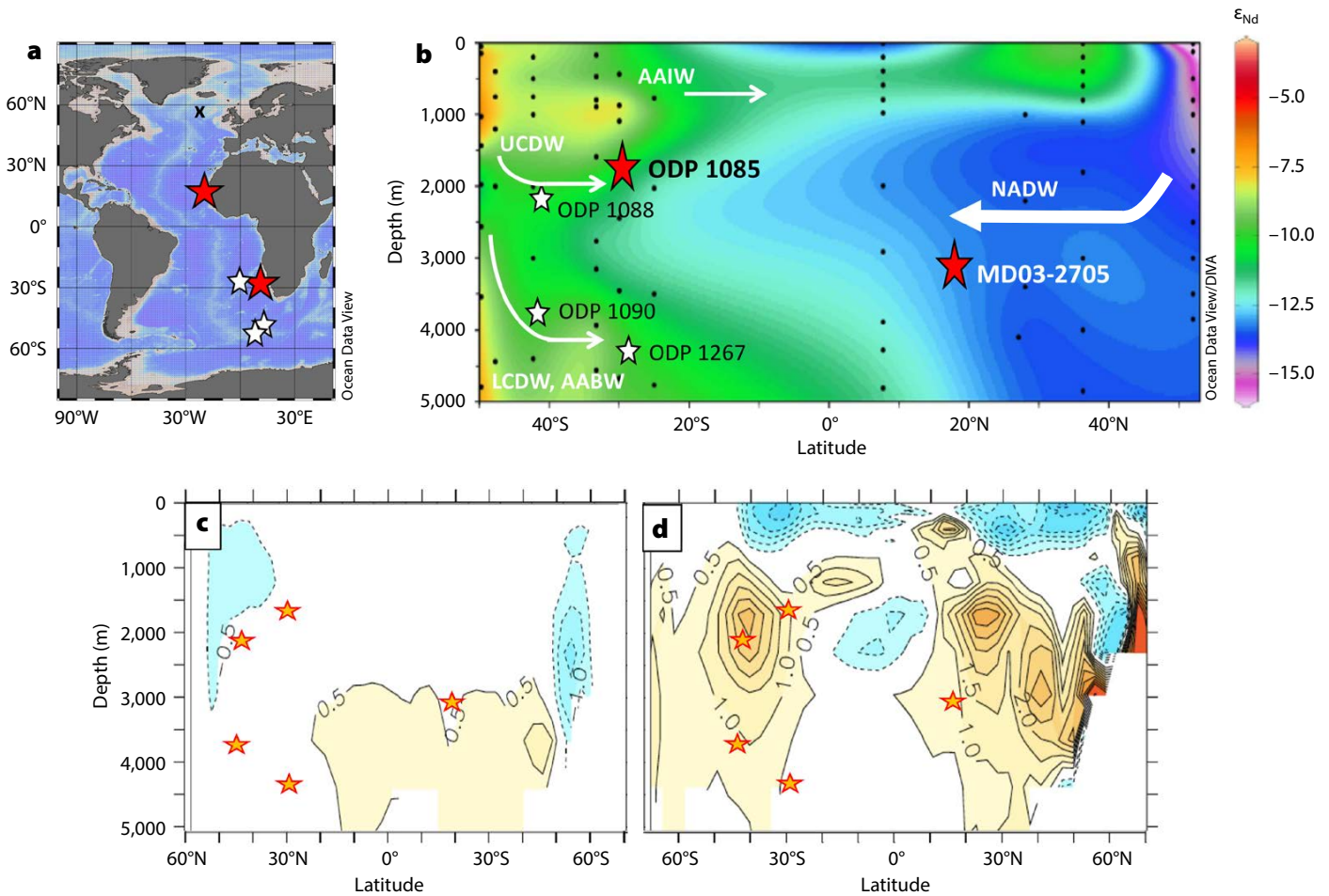
FIGURE 5. Reconstructed seawater \epsilon_{\text{Nd}} records from the eastern Atlantic. (a) Core location map in the Atlantic Ocean. The two red stars indicate cores from MD03-2705 (18°N, 21°W, 3,085 m water depth) and ODP site 1085 (29°S, 14°E, 1,725 m) studied here. The three white stars indicate the sites of previous studies: ODP sites 1088, 1090, and 1267. The black x shows DSDP site 552. (b) Latitudinal transect of present-day seawater \epsilon_{\text{Nd}} values in the Atlantic Ocean (Howe et al., 2016) with the main water masses: NADW = North Atlantic Deep Water; UCDW and LCDW = Upper and Lower Circumpolar Deep Water, AABW = Antarctic Bottom Water, AAIW = Antarctic Intermediate Water. More seawater \epsilon_{\text{Nd}} data are available GEOTRACES IDP2017 ( https://www.bodc.ac.uk/geotraces/data/idp2017/ ). (c) Comparison between reconstructed and zonally averaged simulated seawater \epsilon_{\text{Nd}} anomalies in the case of enhanced southern-sourced water formation. The orange stars mark the sites of reconstructed seawater \epsilon_{\text{Nd}} with positive anomalies at the 900 ka event. Orange and blue shading corresponds to oceanic zones characterized by positive and negative simulated \epsilon_{\text{Nd}} anomalies. (d) The same as (c) in the case of reduced northern-sourced water formation. The simulation results are from Friedrich et al., 2014.
