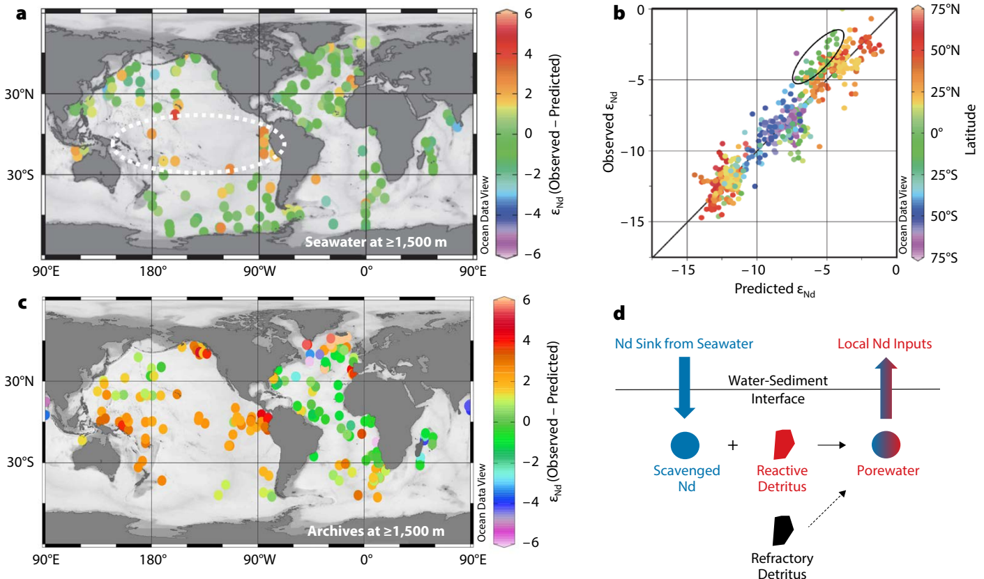
FIGURE 3. Comparison of observed and predicted values for Nd isotopic composition. (a) Spatial distribution of \epsilon_{\text{Nd}} offsets between modern deepwater (≥ 1,500 m depth) and predicted values using empirical equations (Tachikawa et al., 2017). (b) Relationship between measured deepwater Nd isotopic composition and predicted values. (c) Spatial distribution of \epsilon_{\text{Nd}} offsets between archived Holocene (≤10 kyr) sediments and predicted seawater values. (d) Schematic presentation showing the porewater Nd contribution that creates \epsilon_{\text{Nd}} offsets between archival and predicted values. The white dashed ellipse in (a) and the black solid ellipse in (b) indicate the observed \epsilon_{\text{Nd}} offsets in the tropical Pacific. (a), (b), and (c) are adapted from Tachikawa et al. (2017) and (d) is adapted from Du et al. (2016)
