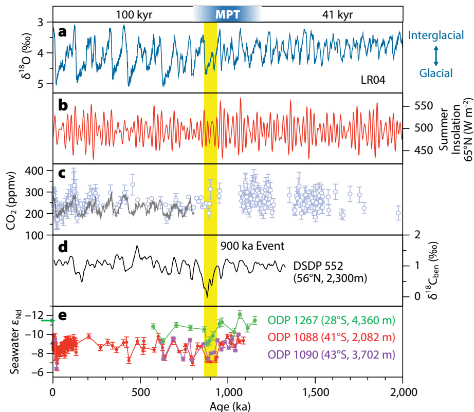
FIGURE 4. Variability across the Mid-Pleistocene transition (MPT). (a) Stack of benthic foraminiferal oxygen isotopic composition ( \delta^{18}\text{O} ) over the last 2 million years (Lisiecki and Raymo, 2005) as an indicator of glacial/interglacial cycles. (b) Summer insolation at 65^\circ\text{N} over the last 2 million years (Laskar et al., 2004). (c) Reconstructed atmospheric \text{CO}_2 concentration (Hönisch et al., 2009; Bereiter et al., 2015; Higgins et al., 2015; Chalk et al., 2017; Dyez et al., 2018). (d) Benthic foraminiferal carbon isotopic composition ( \delta^{13}\text{C} ) record of core from Deep Sea Drilling Project (DSDP) site 552 from the northern Northeast Atlantic ( 56^\circ\text{N} , 23^\circ\text{W} , 2,300 m water depth) over the past 1.3 million years (Raymo et al., 1990) as an example of oceanic \delta^{13}\text{C} changes. (e) Previously published seawater \epsilon_{\text{Nd}} records across the Mid-Pleistocene transition at three sites in the eastern Atlantic: Ocean Drilling Program (ODP) sites 1088 ( 41^\circ\text{S} , 13^\circ\text{E} , 2,080 m) and 1090 ( 43^\circ\text{S} , 9^\circ\text{E} , 3,700 m), and ODP site 1267 ( 28^\circ\text{S} , 2^\circ\text{E} , 4,400 m). Data are from Dausmann et al. (2017); Farmer et al. (2019); Howe et al. (2016); Hu et al., 2016; Pena and Goldstein (2014). The green arrow along the y-axis indicates the present-day seawater \epsilon_{\text{Nd}} value estimated by the empirical equation using temperature and dissolved oxygen concentration (Tachikawa et al., 2017). The yellow band indicates the “900 ka event.”
